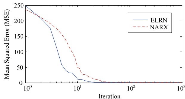
Fig. 5. Training process for neural network thermal models
