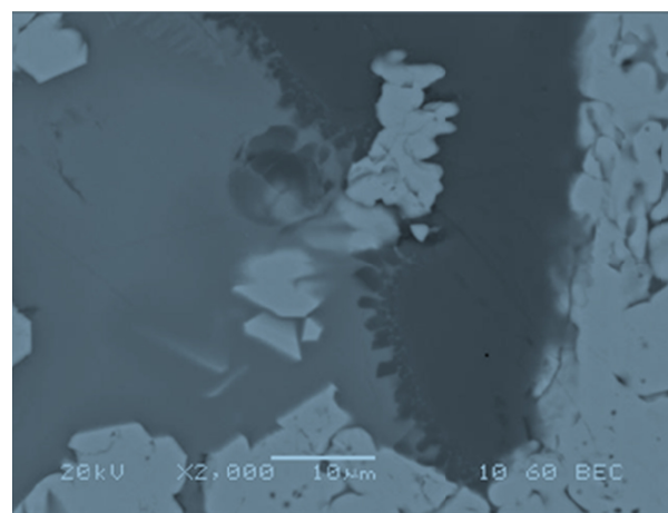
Fig. 3. Microstructure of agglomerate BOR 5 a) hematite, magnetite and calcium ferrites, b) grains area of unsintered and melted mixture
