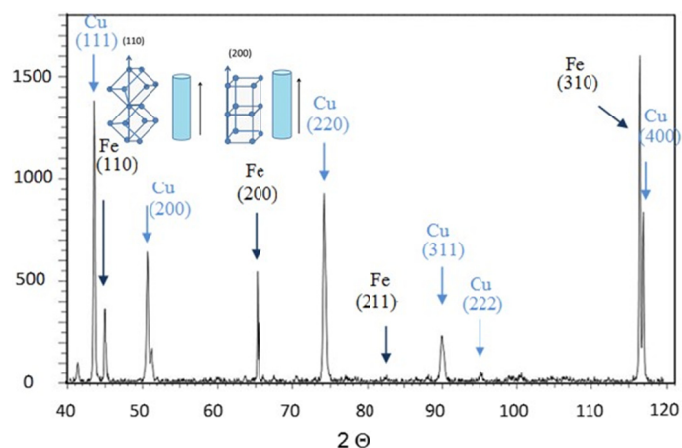
Fig. 3. XRD patterns for the iron nanowire arrays with diameter of 70 nm and length of 3 \mu\text{m} obtained under potential -1.0 V (vs. SHE). The peaks characteristic for the iron and cooper are described with the indices of crystallographic planes
