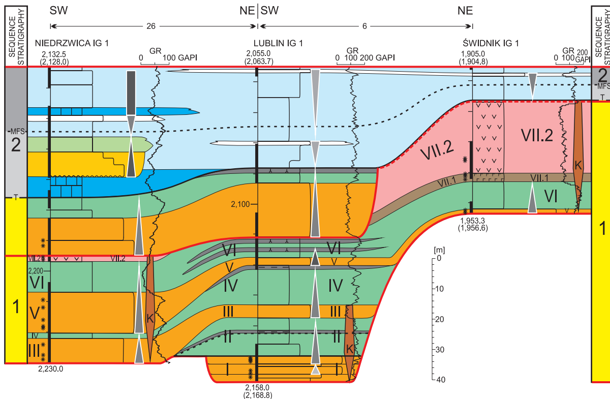
Text-fig. 7. Lithofacies correlation of the Tournaisian and Visean sequences 1 and 2 in the central and SW areas of the Lublin Basin – scheme II; for details see online version.
