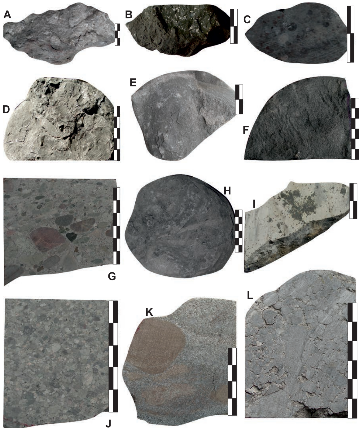
Text-fig. 3. Examples of lithofacies (scale bars = 1 cm): A – Lithofacies L: limestone with nodular structure; borehole Radzyń IG 1; HST of sequence 3; depth 923.50-923.57 m; B – Lithofacies V: basalt with amygdaloidal texture; older lava-flow; borehole Parczew IG 10; sequence 1 – element VII.2; depth 1063.4 m; C – Lithofacies V: heavily altered volcanic rock; borehole Terebin IG 3; sequence 1 – element VII.2; depth 1425.4 m; D – Lithofacies Fm1: massive claystone with bryozoans; borehole Korczmin IG 3; TST of sequence 2; depth 1349.3 m; E – Lithofacies Fm: massive claystone with siderite spherulites; borehole Radzyń IG 1; LST of sequence 4; depth 919.5 m; F – Lithofacies V: basalt; younger lava-flow; borehole Parczew IG 10; sequence 1 – element VII.2; depth 1053.2 m; G – Lithofacies GSm: massive sandy conglomerate; borehole Lublin IG 1; sequence 1 – element I; depth 2157.9 m; H – Lithofacies Fm: massive mudstone with carbonaceous plant chaff; borehole Korczmin IG 1; sequence 1 – element VI; depth 1345.2 m; I – Lithofacies T: tuff; borehole Radzyń IG 1; sequence 1 – element VII.1; depth 941.3 m; J – Lithofacies GSm: massive sandy conglomerate; borehole Niedrzwica IG 1; sequence 1 – element V; depth 2211.9 m; K – Lithofacies GSm: massive sandy conglomerate; borehole Kock IG 2; sequence 1 – element V; depth 1597.8 m; L – Lithofacies Gm: massive sandy conglomerate; borehole Korczmin IG 1; sequence 1 – element V; depth 1347.3 m.
