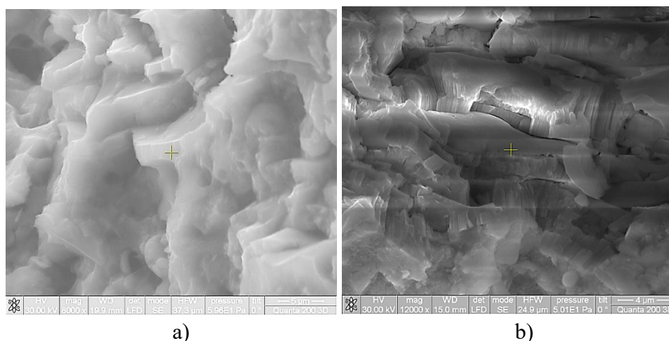
Fig. 5. SE fracture images in case of samples: a) P1 (8.000 \times ), b) P2 (12.000 \times )
