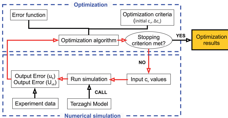
Fig. 2. Flowchart of optimization procedure
