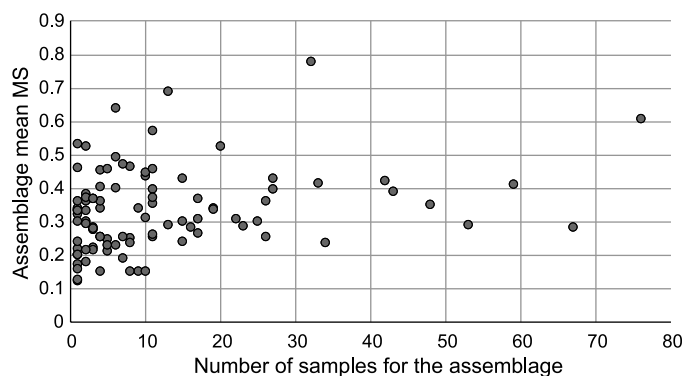
Fig. 2. Mean MS for fossil wood assemblages in studied database as a function of assemblage size, in number of samples measured.
