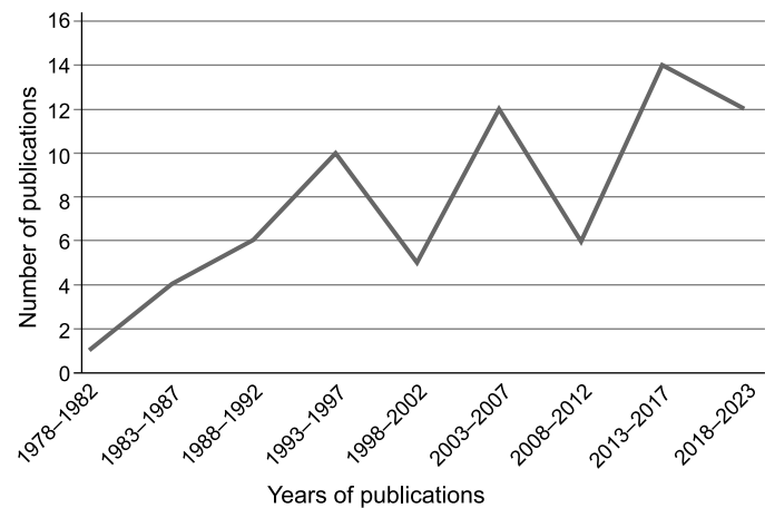
Fig. 1. Number of publications using MS from fossil woods for palaeoclimatological inferences in the database (see SOM).
