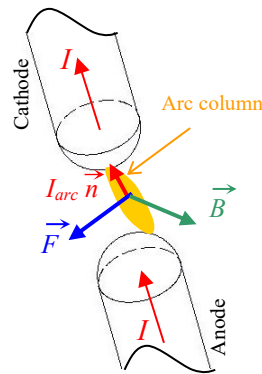
Fig. 10. Magnetic field \vec{B} , electric arc current I_{arc} , and Lorentz force \vec{F} of the arc
