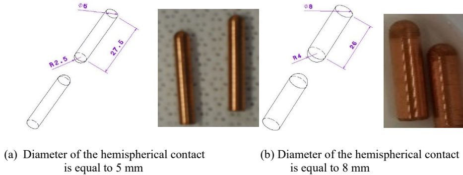
Fig. 1. Dimensions of the used contact samples
