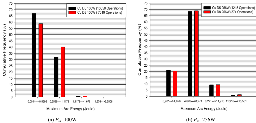
Fig. 6. Histograms of the cumulative frequency versus maximum arc energy for contacts with diameters D=5mm & D=8mm submitted to two input powers
