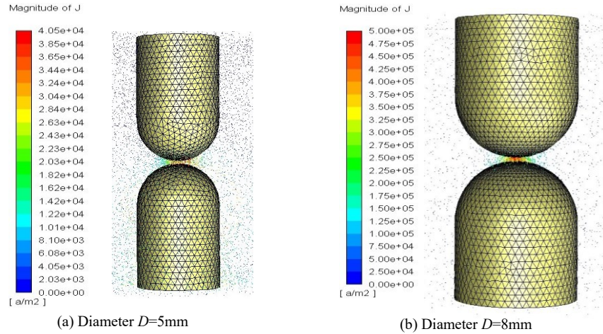
Fig. 11. The distribution of the arc electric current density for the two contacts
