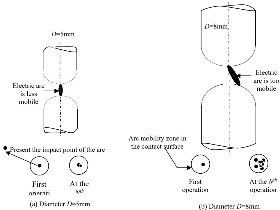
Fig. 12. Arc mobility impact on the degradation of the contact zone of the two contact samples ( D=5\text{mm} & D=8\text{mm} )
