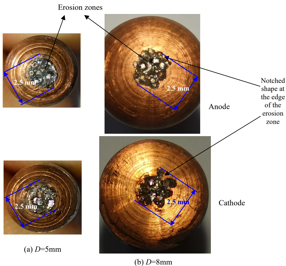
Fig. 9. Erosion of contact surfaces at the end of the lifetime of contacts ( D=5\text{mm} & D=8\text{mm} , P_{in} = 256\text{W} )
