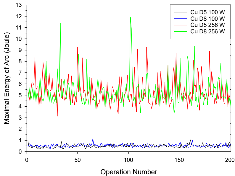
Fig. 5. Maximum arc energy for the two input powers (100W & 256W) and for the two diameters ( D=5\text{mm} & D=8\text{mm} )
