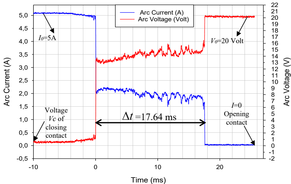
Fig. 3. Arc voltage V_{arc} & arc current I_{arc} for contact opening-closing operation N°300 ( D=5\text{mm} , P_{in}=100\text{W} )
