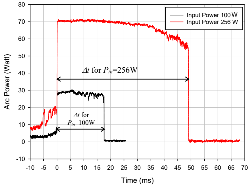
Fig. 4. Arc power for two input powers ( D=5\text{mm} , P_{in}=100\text{W} & 256\text{W} ) (Operation N°300)
