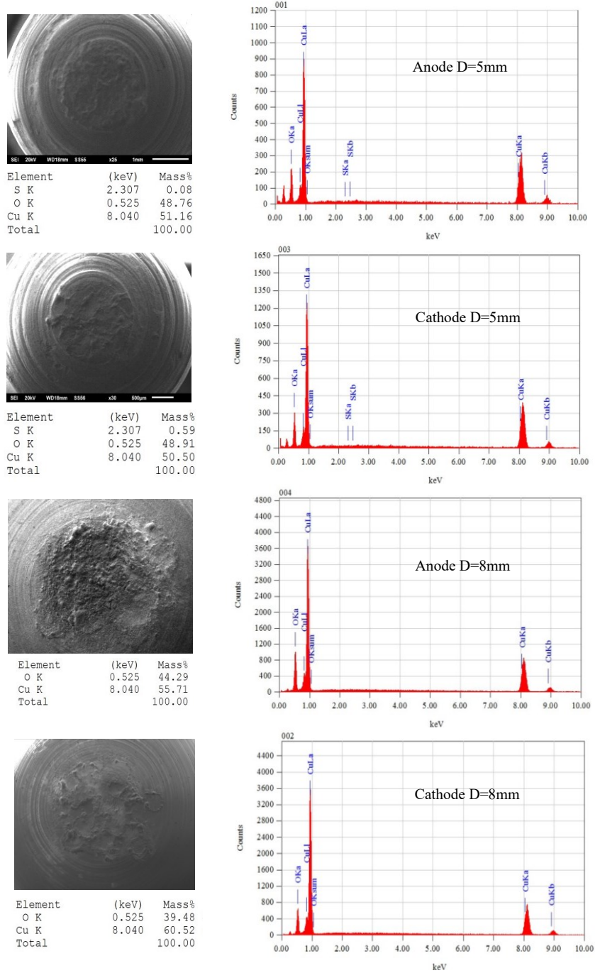
Fig. 7. Scanning Electron Microscopy (SEM) images & Energy dispersive X-ray analysis (EDX) spectra of the chemical composition of the anode and cathode contact surfaces at the end of their lifetime ( P_{in}=256W , D=5mm and 8mm )
