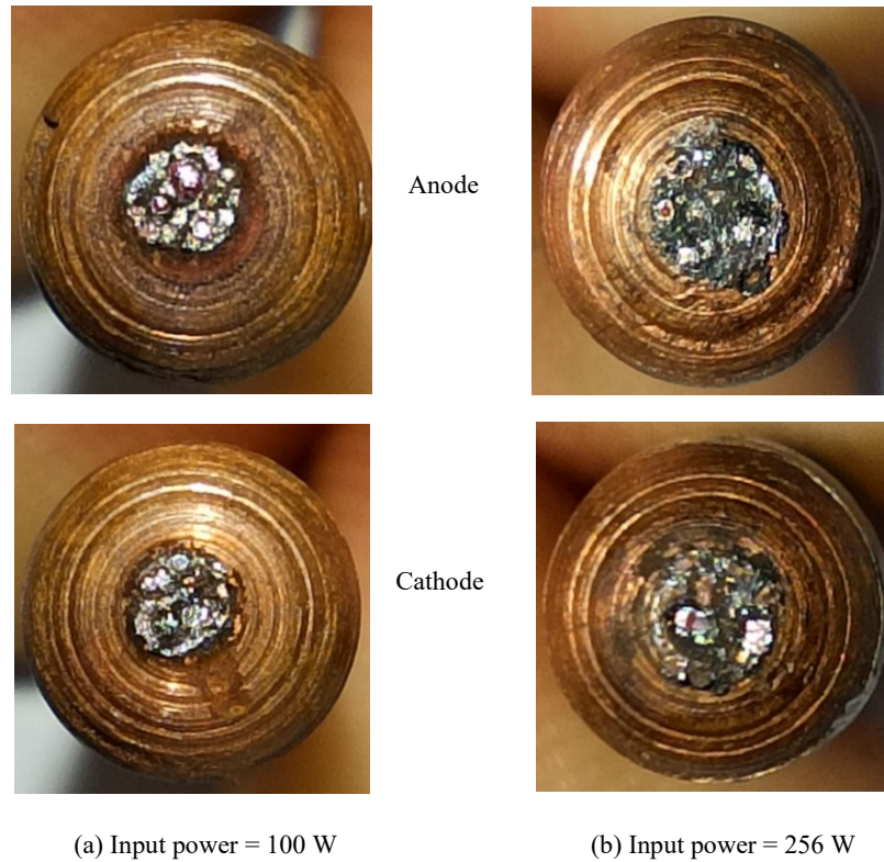
Fig. 8. Erosion of contact surfaces at the end of the contact lifetime (contacts with D=5 mm, P_m=100 W & 256W)
