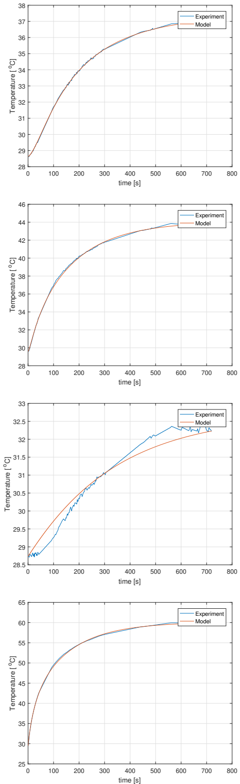
Fig. 5. Step responses of model y^+(k) vs experiments for all areas. Parameters of each model are marked by (F) in tables 2-5. Experimental responses are marked in blue, responses of the model are marked in red.
