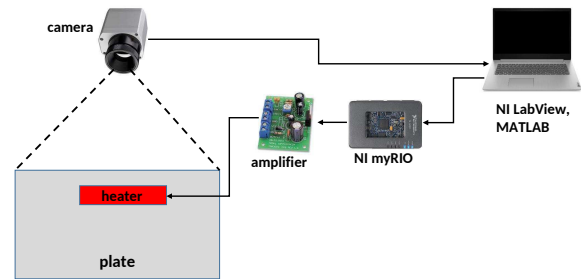
Fig. 2. The construction of the experimental system.
