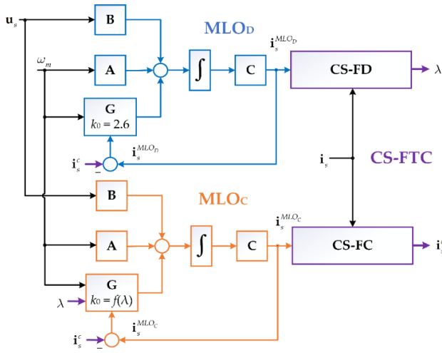
Fig. 7. A scheme of the proposed CS-FTC system.
