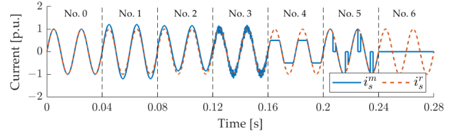
Fig. 2. Waveforms of current for different CS fault types according to Table 1.
