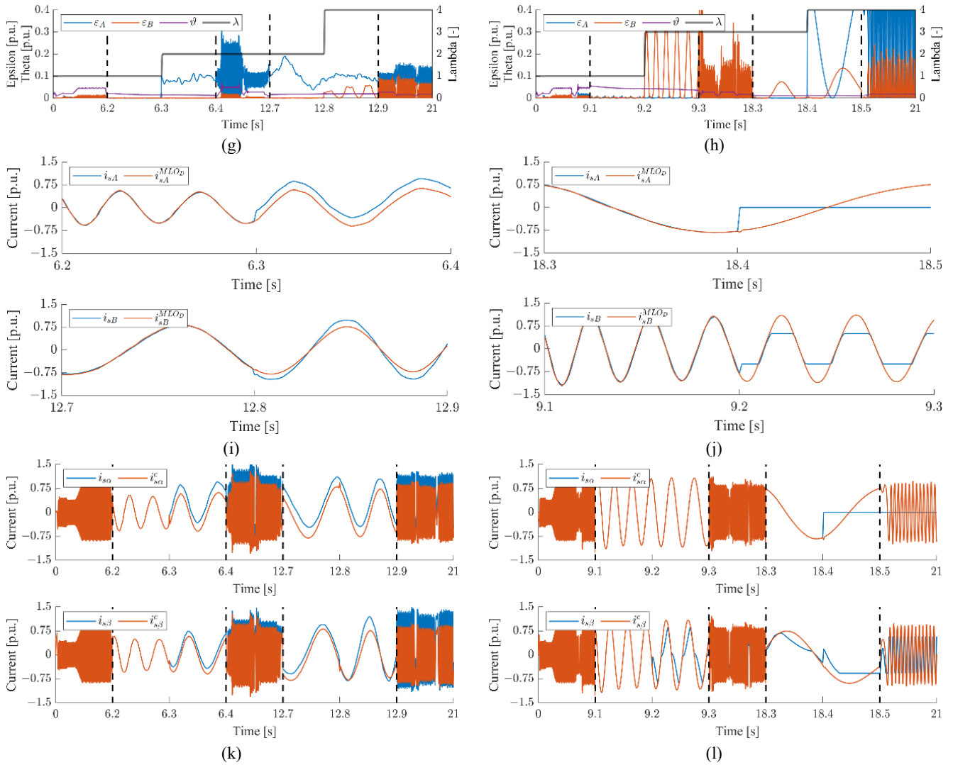
Fig. 11. Waveforms of state variables: speed (a,b), rotor flux (c,d), torque (e,f), coefficients (g,h), and currents used in the detector (i,j), corrected currents; gain and offset (a,c,e,g,i,k), saturation and total signal loss (b,d,f,h,j,l).
