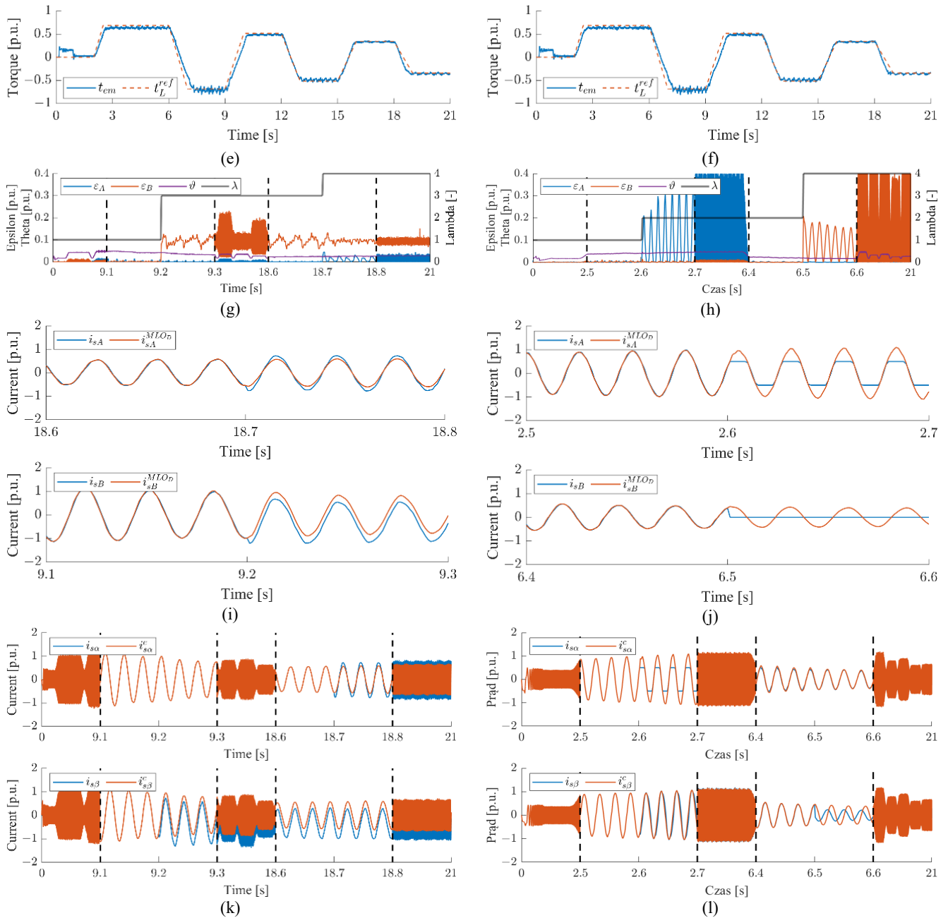
Fig. 12. Waveforms of state variables: speed (a,b), rotor flux (c,d), torque (e,f), coefficients (g,h), and currents used in the detector (i,j), corrected currents; gain and offset (a,c,e,g,i,k), saturation and total signal loss (b,d,f,h,j,l).
