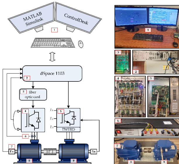
Fig. 8. Diagram of the laboratory set-up.
