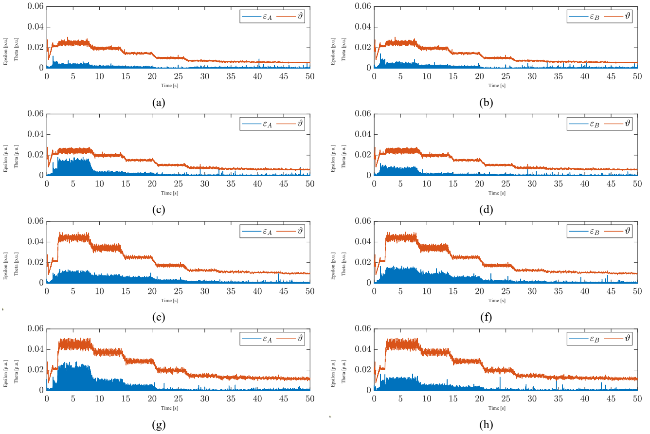
Fig. 10. Waveforms epsilon and theta coefficient in phase A (a,c,e,g) and B (b,d,f,h) for motoring (a,b,e,f) and regenerating (c,d,g,h) operations, 25% of the rated load (a,b,c,d) and 75% of the rated load (e,f,g,h).
