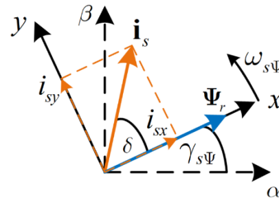
Fig. 3. Idea of DFOC method – vector diagram.
