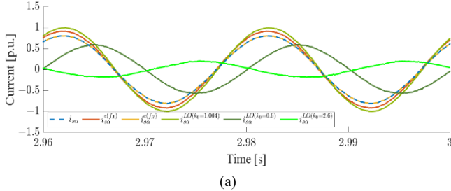
Fig. 5. Waveforms of \alpha (a) and \beta (b) stator current components for different estimation methods.
