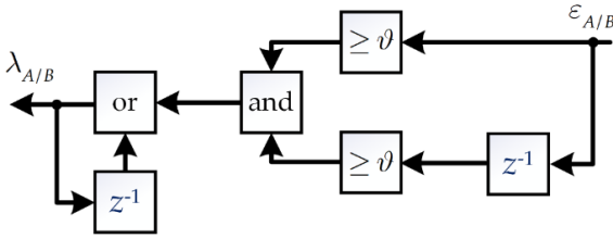
Fig. 6. A scheme of the proposed CS-FD system.
