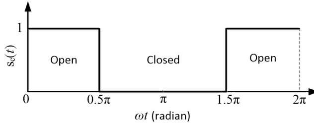
Fig. 4. Variation of crack switching function, s_c(t) with shaft rotation [53]
