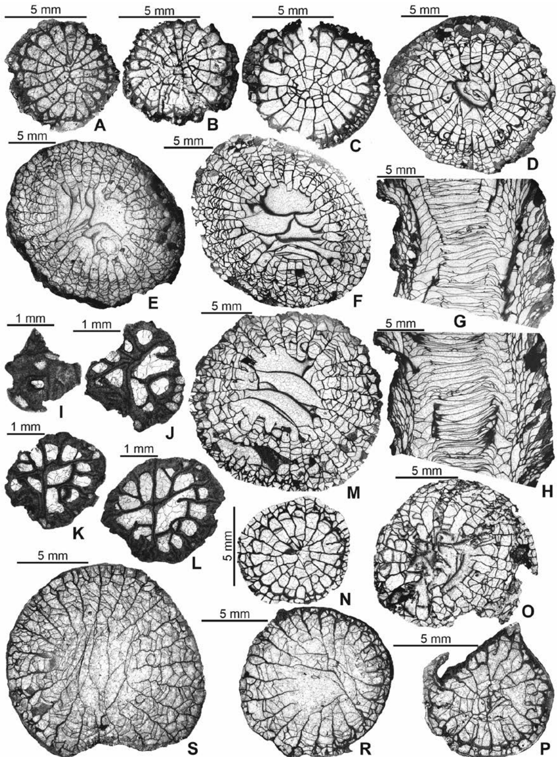
Text-fig. 12. Yvanophylloides (Patulaxis) parvus sp. nov. Transverse sections, except when stated otherwise. A–H – USNM PAL 795385, holotype; A, B – late neanic growth stage, C – late neanic/early mature growth stage, D–F – successive sections of mature growth stage, G, H – longitudinal sections; G – slightly eccentric, H – centric. I–M – USNM PAL 795386; I–L – neanic growth stage, M – mature growth stage. N, O – USNM PAL 795387; N – late neanic/early mature growth stage, O – mature growth stage. P–S – USNM PAL 795388; P – late neanic/early mature growth stage, R – early mature growth stage, S – mature growth stage. For stratigraphic positions see text.
