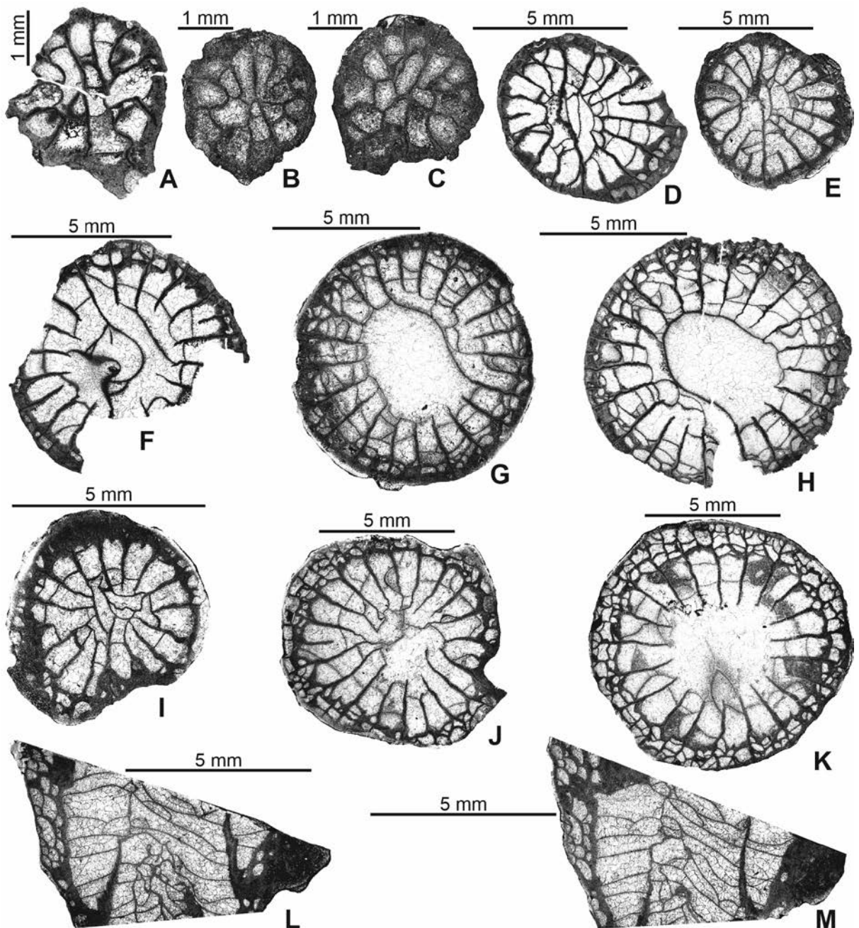
Text-fig. 15. Yuanophylloides (Patulaxis) sp. Transverse sections, except when stated otherwise. A–H – USNM PAL 795401; A–C – neanic growth stage, D, E – late neanic/early mature growth stage, F–H – mature growth stage; I–M – USNM PAL 795402; I – late neanic/early mature growth stage, J, K – mature growth stage, L, M – longitudinal sections; L – eccentric, M – almost centric. For stratigraphic positions see text.
