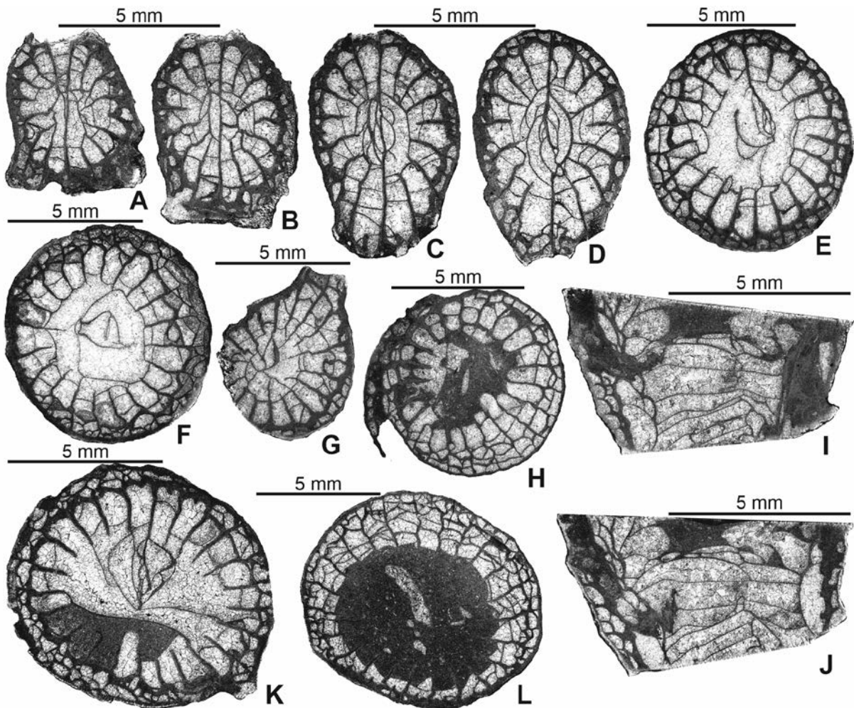
Text-fig. 7. Yuanophylloides (Yuanophylloides) perplexus (Cocke, 1970). Transverse sections, except when stated otherwise. A–F – USNM PAL 795349; A–C – neanic growth stage, D – late neanic/early mature growth stage, E, F – mature growth stage. G–J – USNM PAL 795350; G – neanic growth stage, H – mature growth stage, I, J – longitudinal sections; I – centric, J – slightly eccentric. K, L – USNM PAL 795351; K – mature growth stage, L – calice reduced in size. For stratigraphic positions see text.
