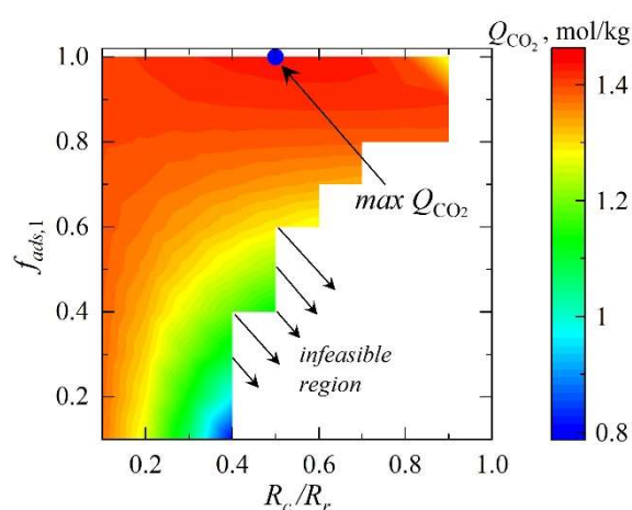
Figure 7. Objective function, Q_{CO_2} , for optimizing the structure of nonadiabatic bed with the radially nonuniform distribution of adsorbent, comprising two decision variables, i.e., core radius, R_c , and volume fraction of sorbent particles in the core, f_{ads,1} , together with its maximum (denoted with bullet). Optimization was done by setting T_w = 298.15 K and the adsorbent-to-catalyst ratio equal to 5:1.
