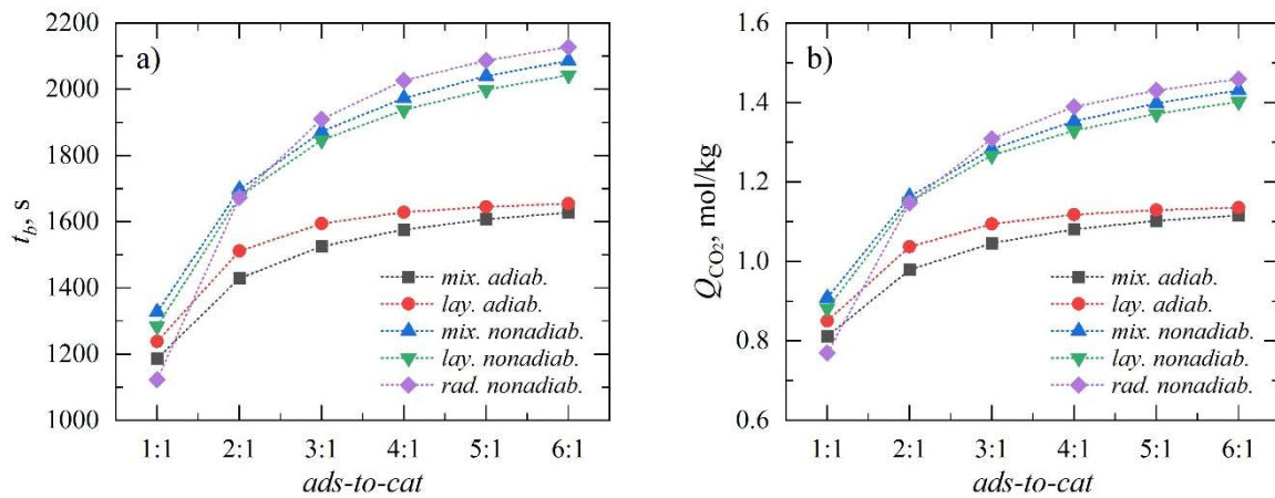
Figure 8. Bed breakthrough time, t_b (a), and corresponding values of the average adsorbate concentration in the sorbent, Q_{CO_2} (b), determined for different configurations of hybrid bed depending on adsorbent-to-catalyst ratio, where mix. denotes a bed made of uniform mixture of particles, lay. corresponds to a bed made of six alternating layers, and rad. denotes bed with optimal radially nonuniform distribution of adsorbent.
