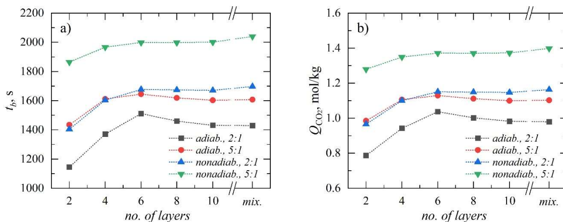
Figure 4. Bed breakthrough time, t_b (a), and corresponding values of the average adsorbate concentration in the sorbent, Q_{CO_2} (b), determined for adsorbent-to-catalyst ratios equal to 2:1 and 5:1, for both adiabatic and nonadiabatic ( T_w = 298.15 K) bed vs. number of alternating layers.
