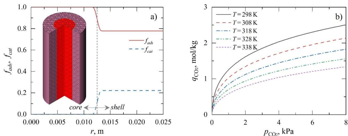
Figure 3. Radial distributions of adsorbent and catalyst volume ratio in configuration with the radially nonuniform sorbent distribution (a), and adsorption isotherms of CO 2 on zeolite 13X (b) determined for different temperatures based on parameters from Wang and LeVan (2009).
