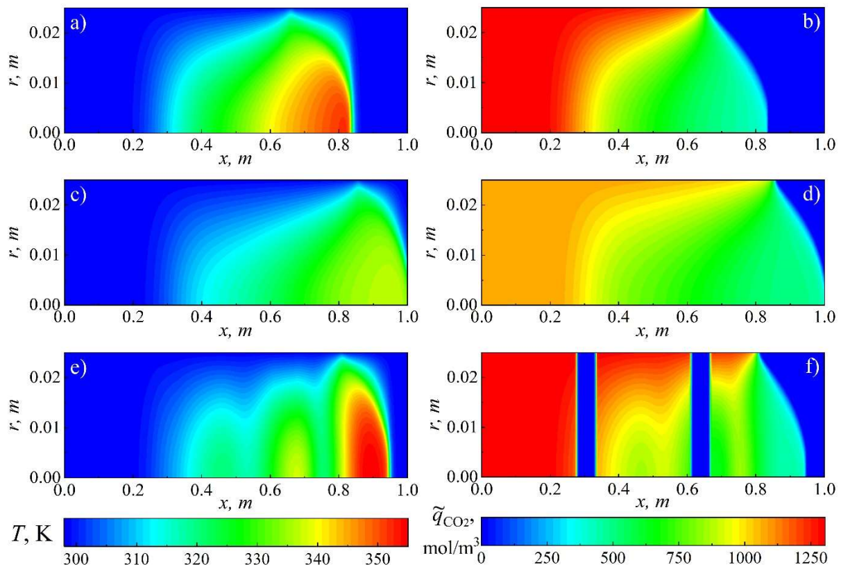
Figure 6. Spatial distributions of temperature (left column) and solid-phase concentration of \text{CO}_2 (right column) expressed in moles per cubic meter of hybrid reactor at t_b for: (a)–(b) bed with two layers ( t_b = 1864.93 \text{ s} ), (c)–(d) bed made of uniform mixture of particles ( t_b = 2039.97 \text{ s} ), and (e)–(f) bed with six layers ( t_b = 1999.36 \text{ s} ). In all cases, the bed is nonadiabatic ( T_w = 298.15 \text{ K} ), and adsorbent-to-catalyst ratio is 5:1.
