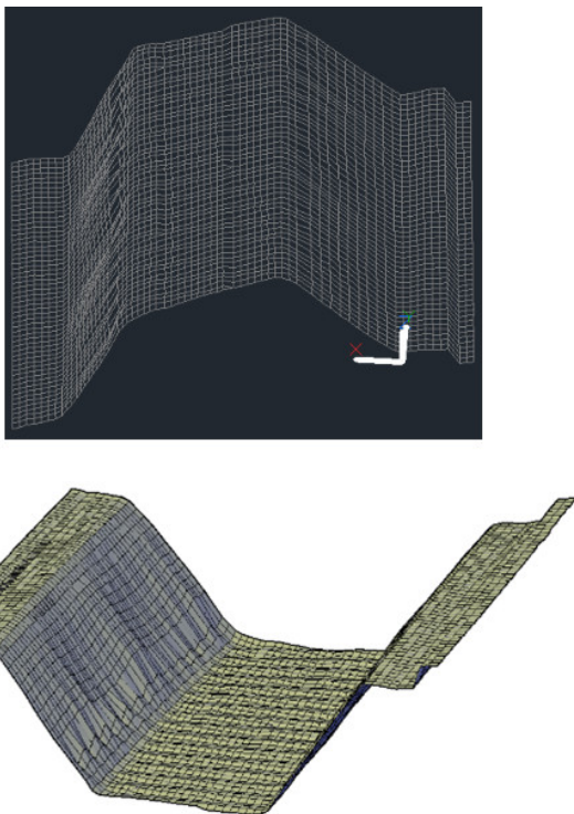
Fig. 11. UBM 240 panel – result of scanning by Leica 3D Disto
