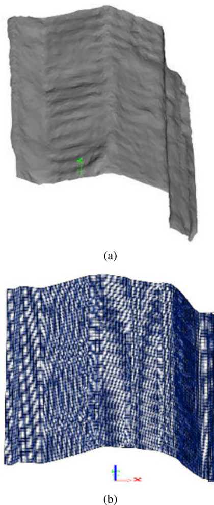
Fig. 14. FEM models of UBM panels in SCIA Engineer: (a) based on MagiScan model; (b) based on Leica model
