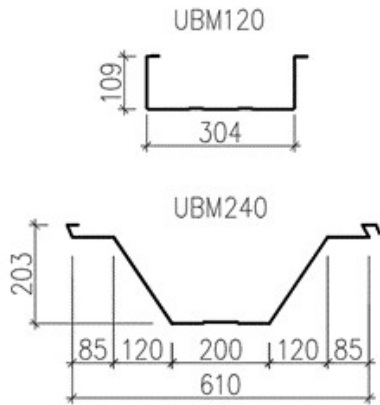
Fig. 2. Cross-sections of the UMB profiles
