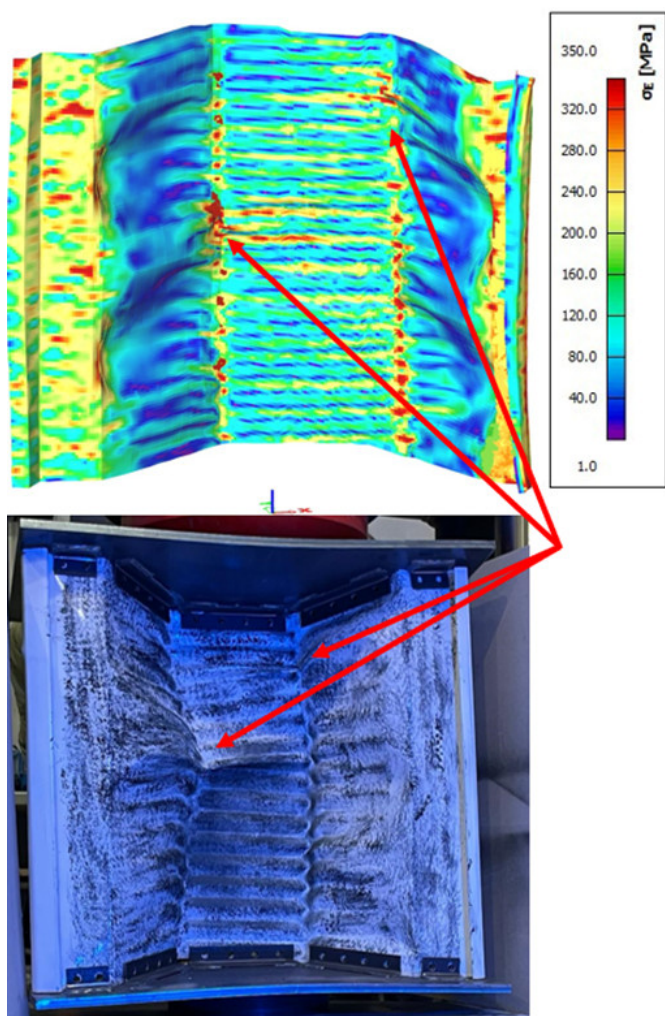
Fig. 19. Failure deformations: numerical, experimental
