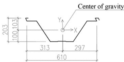
Fig. 16. Centre of gravity for UBM 240 profile ( t = 1.00 mm)
