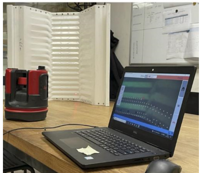
Fig. 10. 3D scanning of corrugated UBM 240 panel
