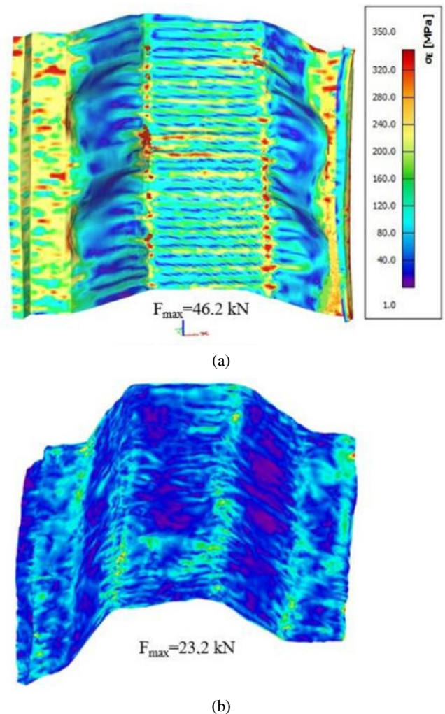
Fig. 15. Misses stresses distribution and deformations for ultimate load: (a) for model basis on Leica geometry; (b) for model basis on MagiScan model
