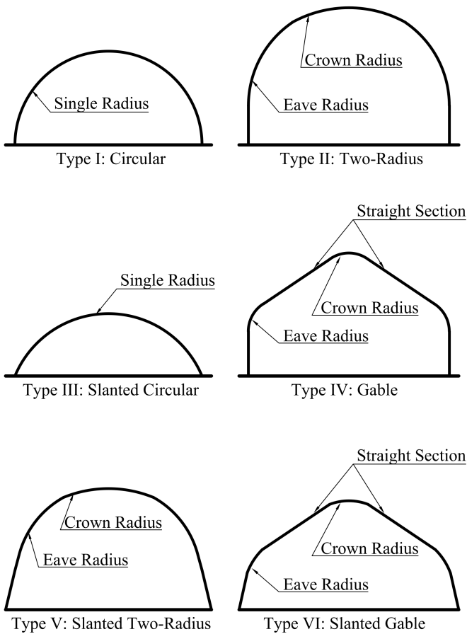
Fig. 1. Possible UMB buildings shapes
