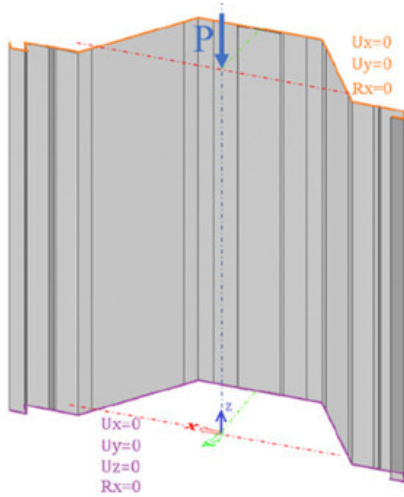
Fig. 13. Panel load and boundary conditions
