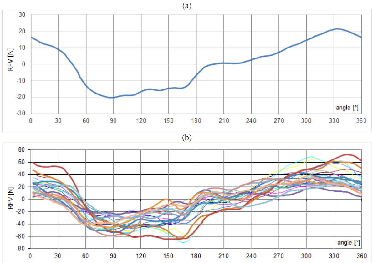
Fig. 9. Reference specification: a) average waveform; b) partial waveforms.
