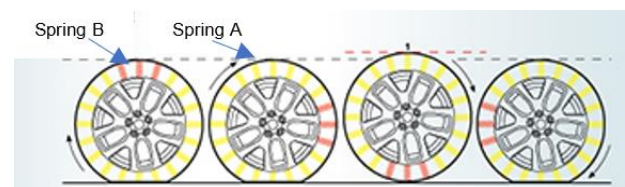
Fig. 6. Radial force variation spring model [35].
