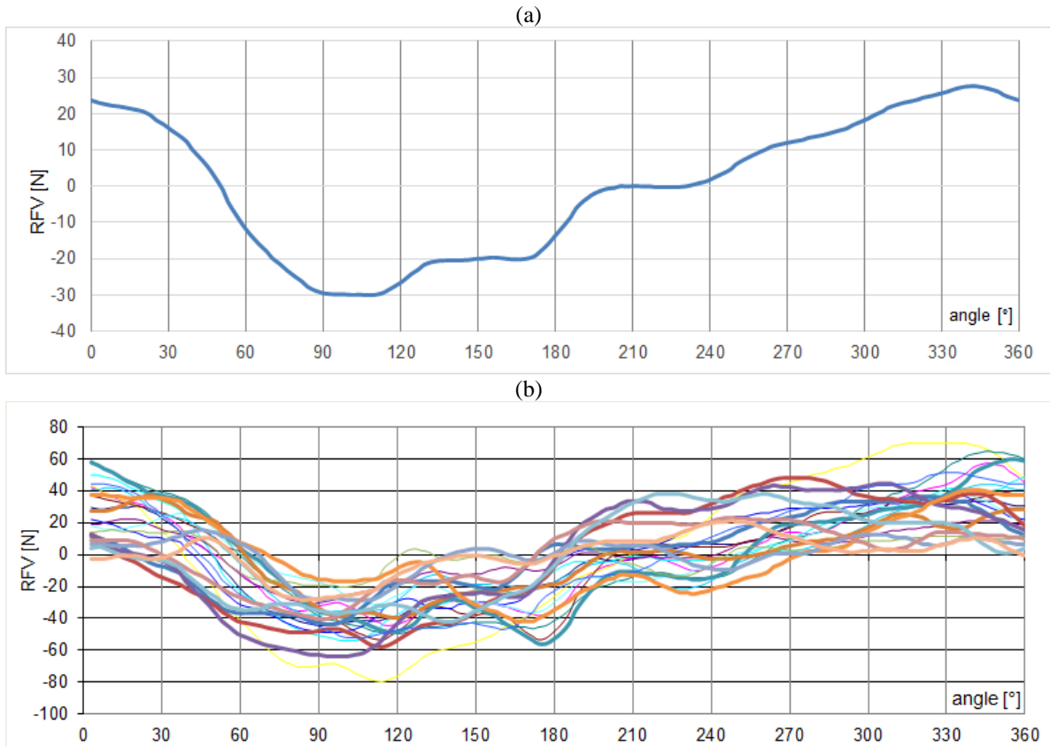
Fig. 11. Shaping drum factor: a) average waveform; b) partial waveforms.
