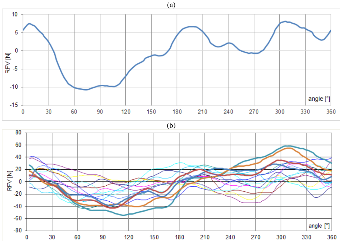
Fig. 13. B&T drum: a) average waveform; b) partial waveforms.
