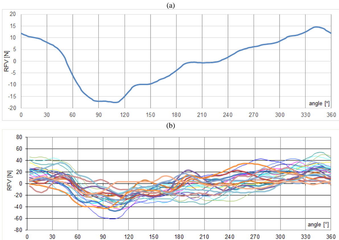
Fig. 14. Reference parameters recovery: a) average waveform; b) partial waveforms.
