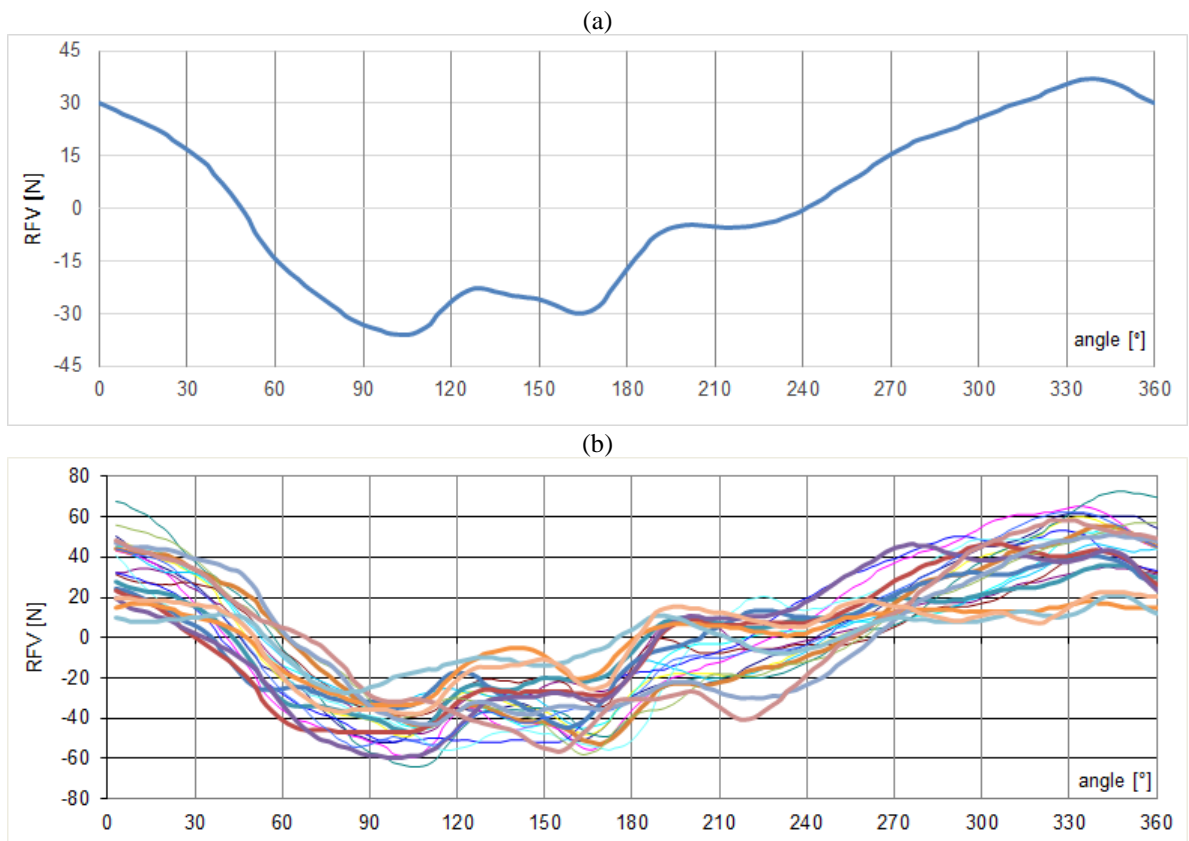
Fig. 10. Carcass transfer ring factor: a) average waveform; b) partial waveforms.
