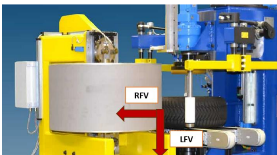
Fig.5. Tire uniformity measuring drum [32]
