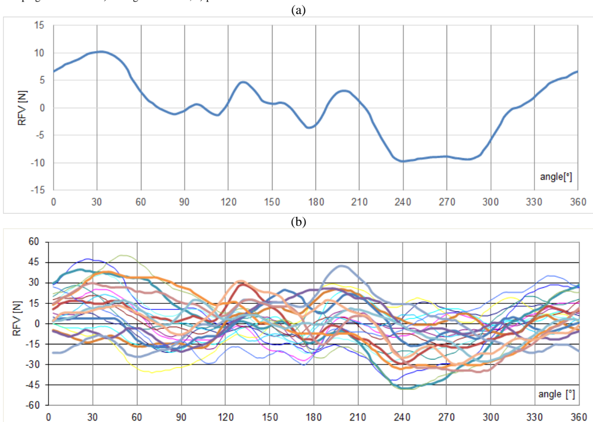
Fig. 12. B&T transfer ring factor: a) average waveform; b) partial waveforms.
