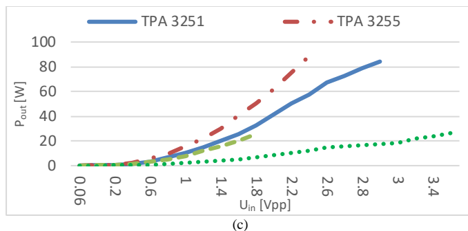
Fig. 4. Output power of the power amplifiers for (a) 2.2 Ω (b) 3.9 Ω (c) 4.7 Ω load
