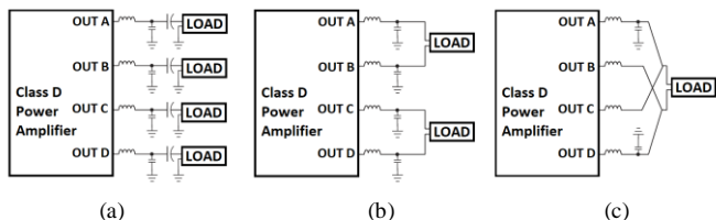
Fig. 1. Output configurations of the selected power amplifiers (a) 4 channel single-ended (b) 2 channel-bridge-tied load (c) 1 channel-parallel bridge-tied
