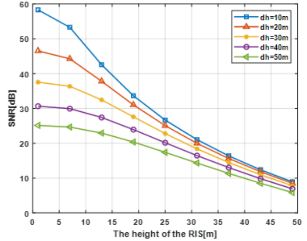
Fig.3. SNR varying with the height of RIS.
