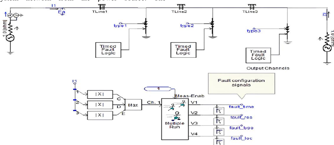
Fig. 2. Transmission line model [22]
