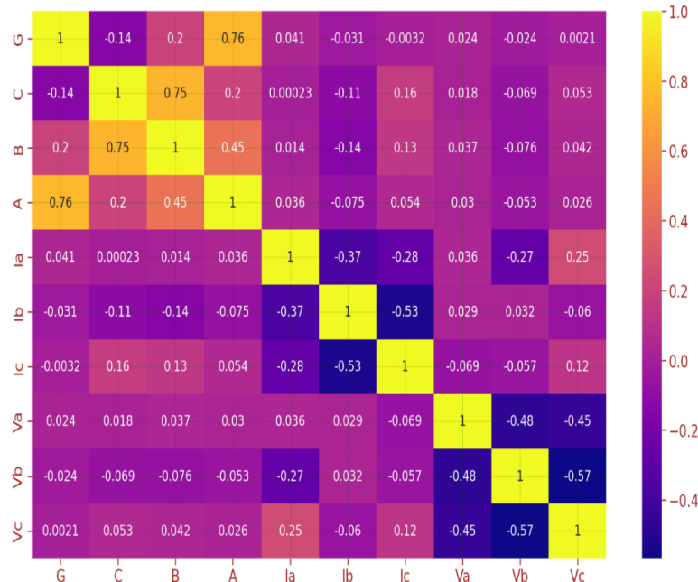
Fig. 3. Correlation matrix
