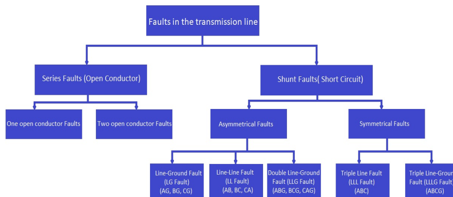
Fig. 1. Classification of fault types in transmission line [3]
