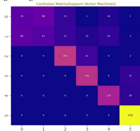
Fig. 6. Confusion matrix of SVM
