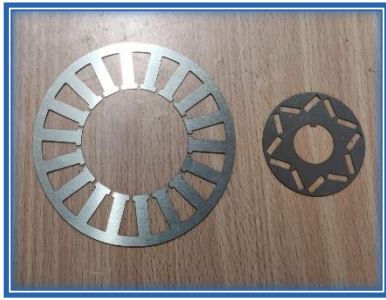
Fig. 3. Laminated Stator and Rotor developed motor
