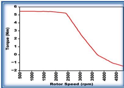
Fig. 6. Speed -Torque characteristics of motor
