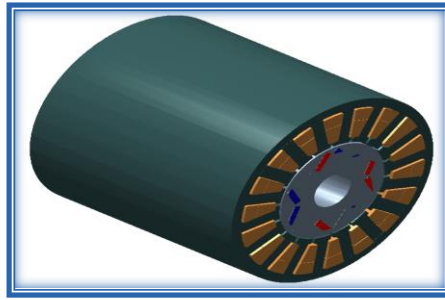
Fig. 4. 3D view of the motor using motor solve software
