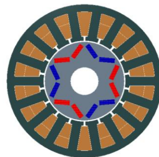
Fig. 2. Structure of 6 poles, 18 slots BLDCM with the inner rotor
