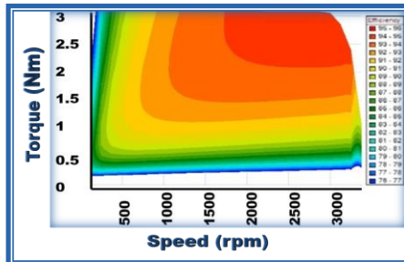
Fig. 7. Efficiency contour of the BLDC motor
