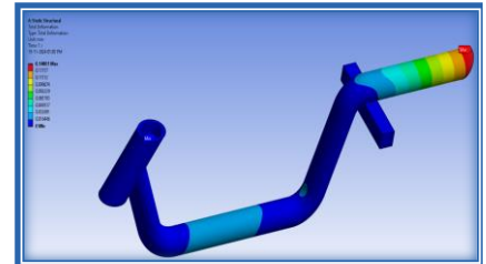
Fig. 14. Total deformation
