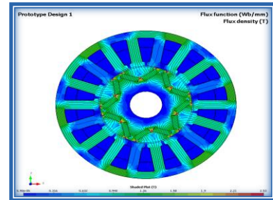
Fig. 8. Magnetic saturation of the designed motor
