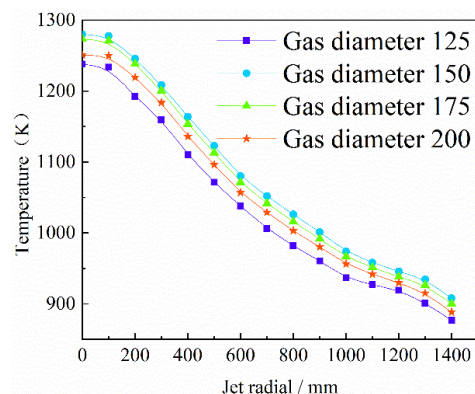
Fig. 16. Bottom centerline temperature for different nozzle spacings
