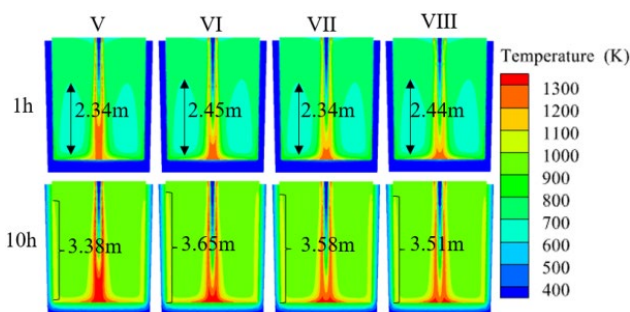
Fig. 13. Temperature field distribution for different nozzle spacing
