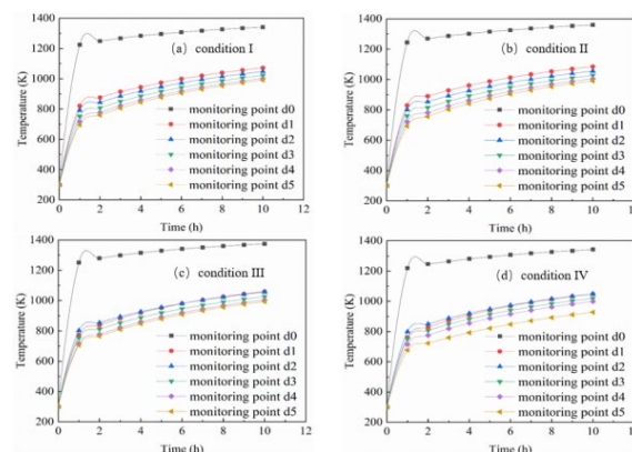
Fig. 12. Temperature line graph of monitoring points
