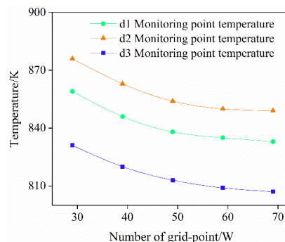
Fig. 3. Verification of grid-independence
