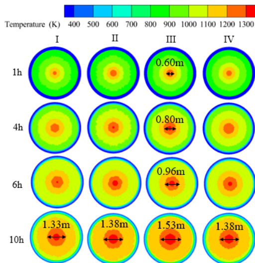
Fig. 10 Contour plot of bottom temperature distribution at different fuel gas velocities
