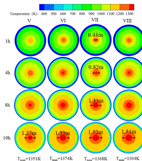
Fig. 14. Temperature distribution of the bottom disk for different nozzle spacing
