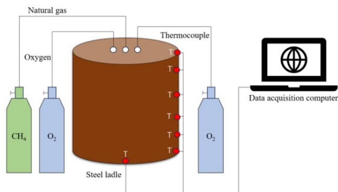
Fig. 4 Schematic diagram of the experiment
