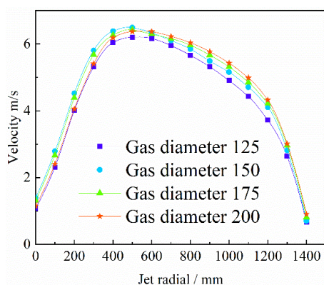
Fig. 15. Bottom centerline velocity for different nozzle spacings
