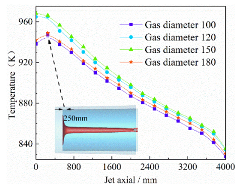
Fig. 11. Radial temperature of the inner wall surface over 4h at different fuel gas velocity
