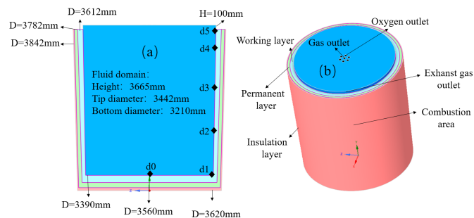
Fig. 1. Schematic diagram of ladle structure (a) Dimensional structure (b) Computational geometric modeling
