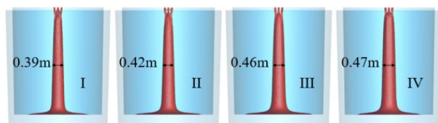
Fig. 5. Comparison of flame shapes under different fuel gas velocities
