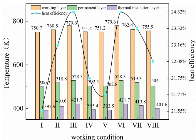
Fig. 18. Final Average Temperature and Thermal Efficiency of Inner and Outer Walls
