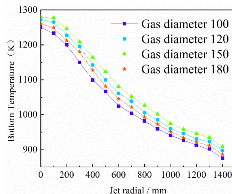
Fig. 9. Bottom centerline temperature
