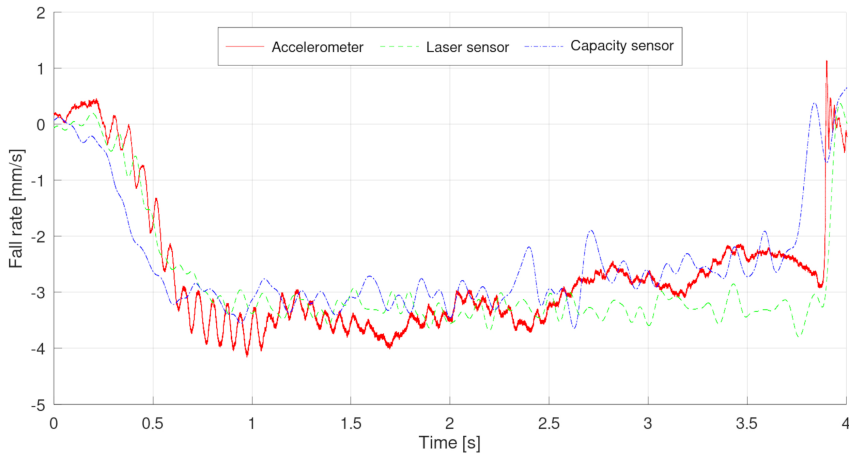
Fig. 4. Comparison of fall rate data gathered by the accelerometer, laser sensor, and capacity sensor.
