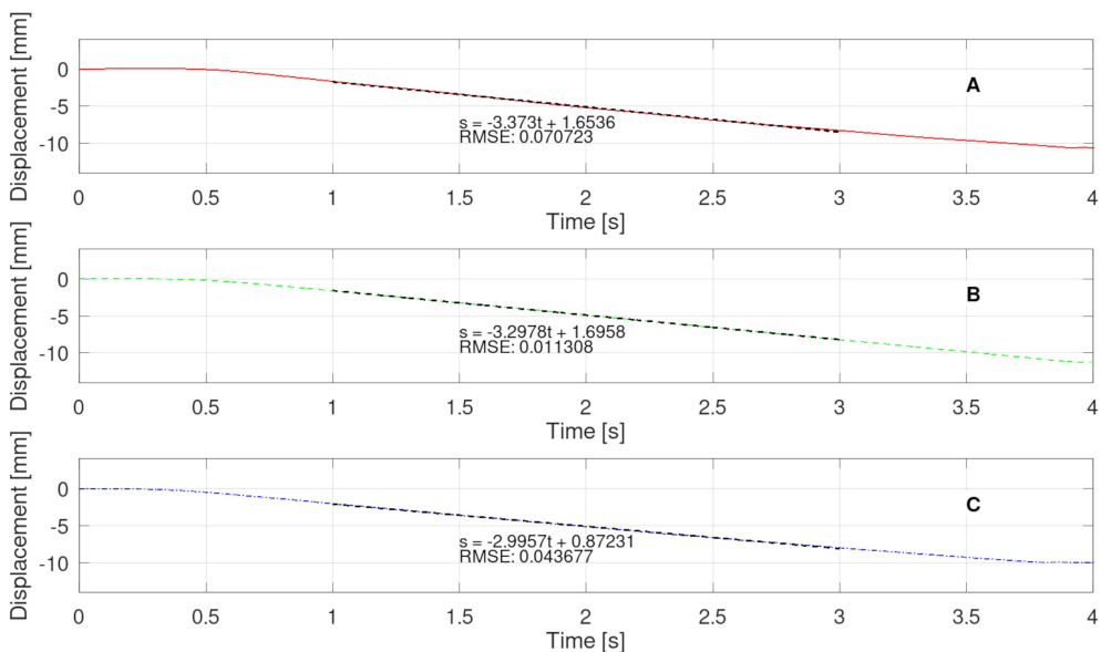
Fig. 5. Trend lines computed for every sensor’s characteristics (displacement): A – accelerometer, B – laser sensor, C – capacity sensor.
