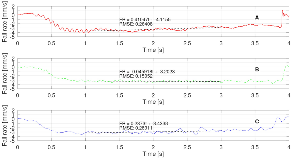
Fig. 6. Trend lines computed for every sensor's characteristic (fall rate): A – accelerometer, B – laser sensor, C – capacity sensor.
