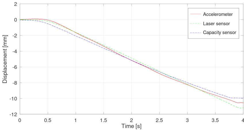
Fig. 3. Comparison of displacement data gathered by the accelerometer, laser sensor and capacity sensor.
