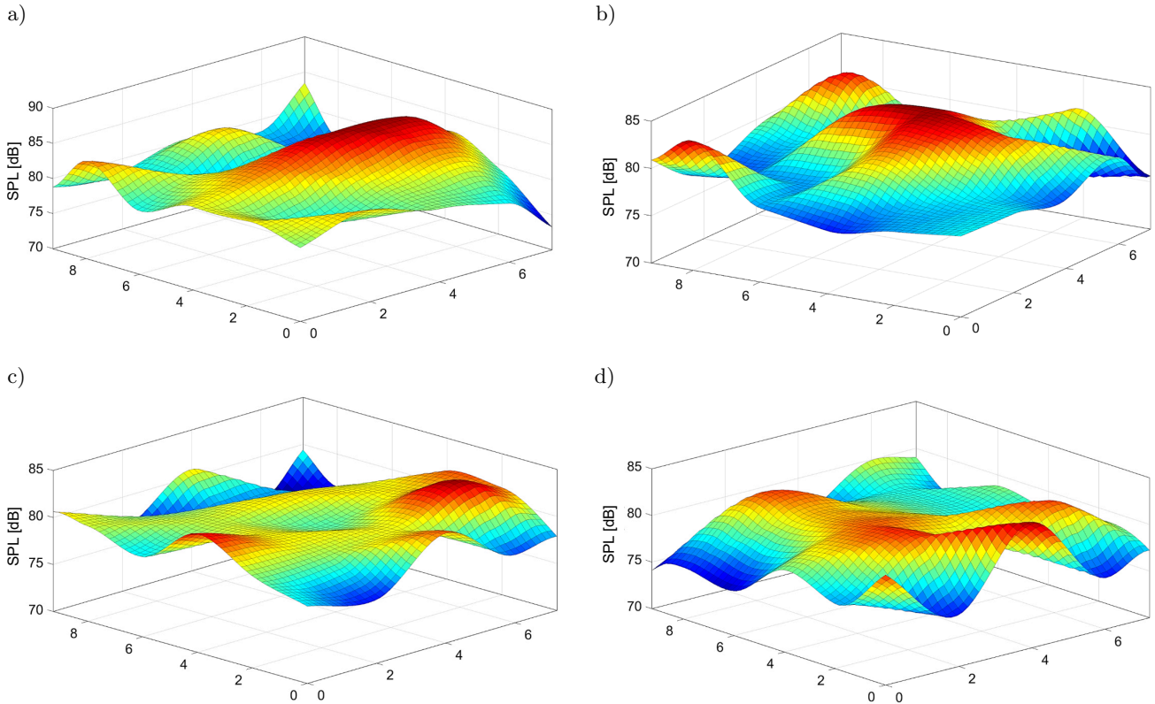
Fig. 7. Variation in SPL at the third fixed position of the source in: (a) plane 1; (b) plane 2; (c) plane 3; (d) plane 4.
