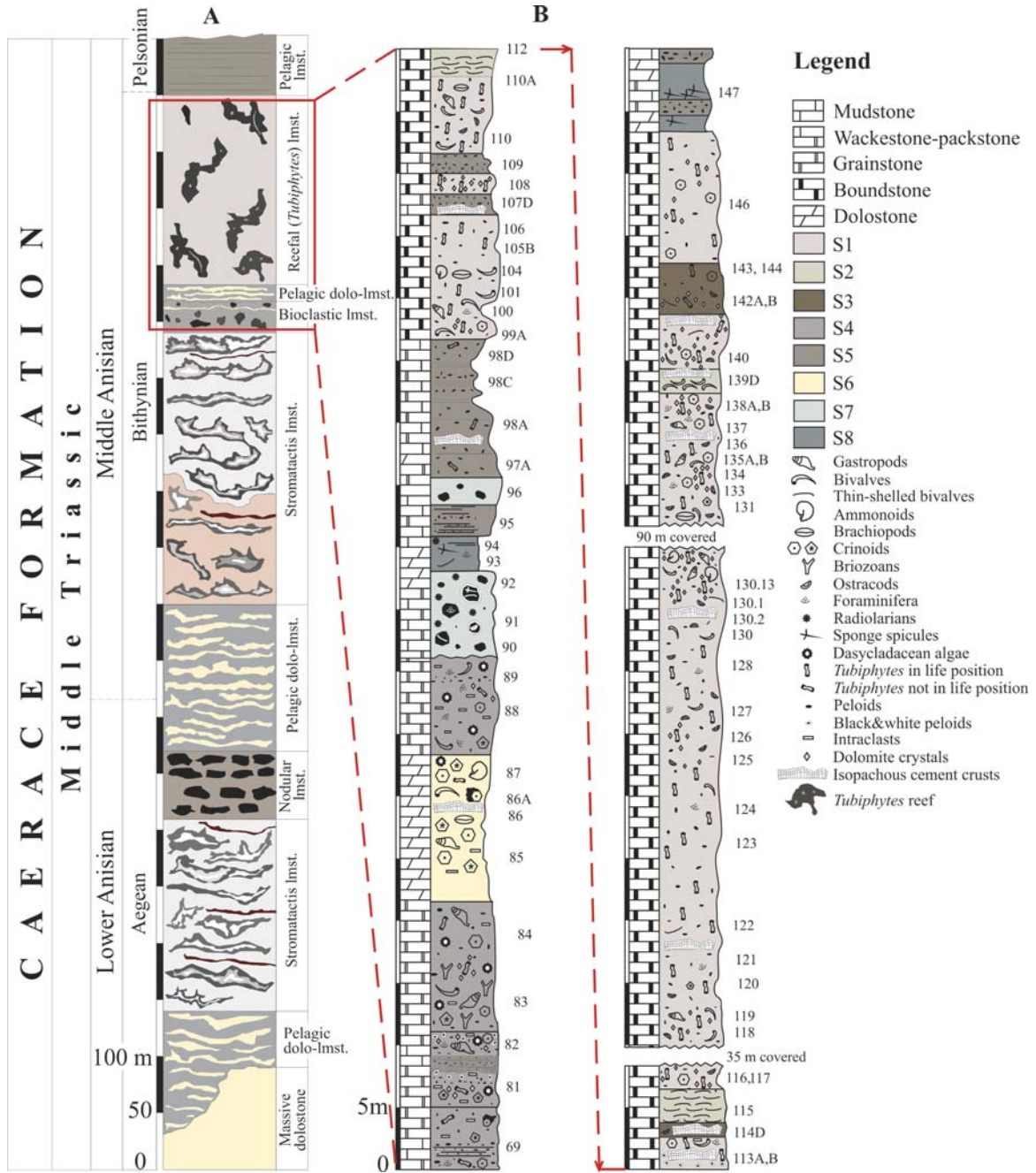
Text-fig. 4. Synthetic lithological column (A) of the Middle Anisian Caerace Formation in the Mahmudia Quarry, and detailed lithofacies column (B continued) of the studied section (marked by the red quadrangle) with sample log for the lower Middle Anisian (Bithynian) Tubiphytes -buildup. Symbols S1 to S8 as shown in Text-fig. 3 and Table 1
