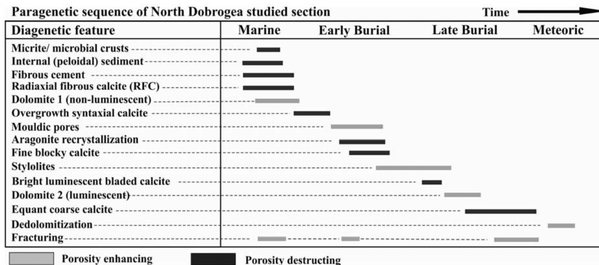
Text-fig. 7. Schematic representation of the diagenetic history of the lower Middle Anisian section of the Caerace Formation in the Mahmudia Quarry. Note the difference between porosity-destructing and porosity-enhancing factors
