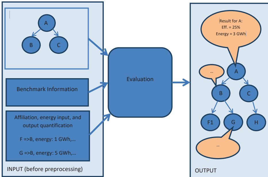
Fig. 15. Algorithm overview—inputs and outputs (General Form)
