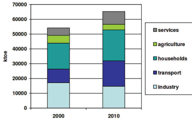
Fig. 10. Final energy consumption by sector in Poland in 2000 and 2010 Source: (Central Statistic Office 2012: 7). 8
