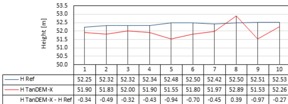
Fig. 12. Height values of terrain profile points and points interpolated from the IDEM
