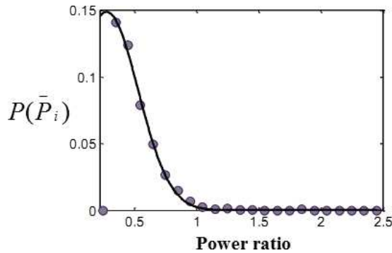
Fig. 3. Probability of the phoneme with a given energy (a) or power ratio (b) to be the last in the sentence.
