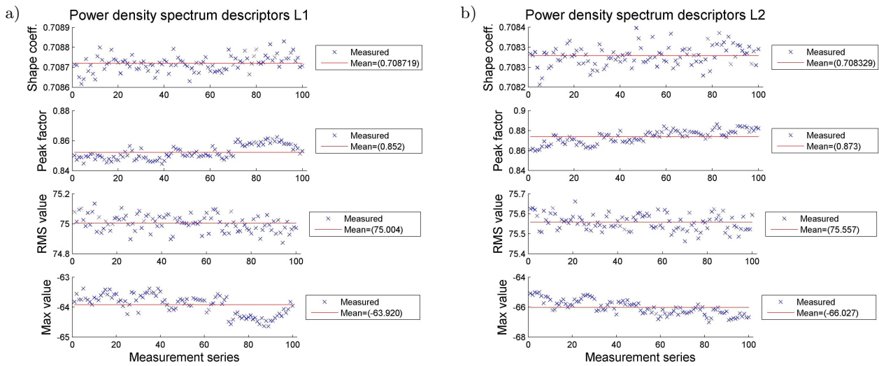
Fig. 16. Power density spectrum descriptors collective results of AE signals generated by PD source inside the electrical power transformer: a) for sensor over L1 phase, b) for sensor over L2 phase.
