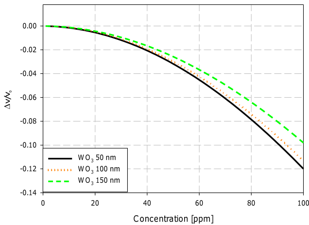
Fig. 7. SAW velocity changes on CO vs. concentration from 0 to 100 ppm in synthetic air in the case of three sensor layers \text{WO}_3 (50, 100, 150 nm) in T = 40^\circ\text{C} . Calculations were performed for: the sensitivity coefficient a = 0.5 \text{ ppm}^{-1} , \sigma_S = 4.7 \times 10^{-7} \text{ S} , k = 10^8 \text{ s}^{-1} , D_K = 10^{12} \text{ nm}^2 \text{ s}^{-1} , E_g = 2.7 \text{ eV} , M = 28 \text{ g/mol} , r = 2 \text{ nm} (CO).
