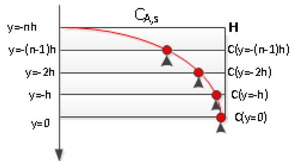
Fig. 2. Iteration takes into consideration the gas concentration in the next sub-layer SAW sensor.
