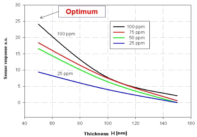
Fig. 6. Influence of the thickness of the \text{WO}_3 layer on the response of carbon monoxide vs. concentration: 25, 50, 75, 100 ppm) in T = 40^\circ\text{C} .
