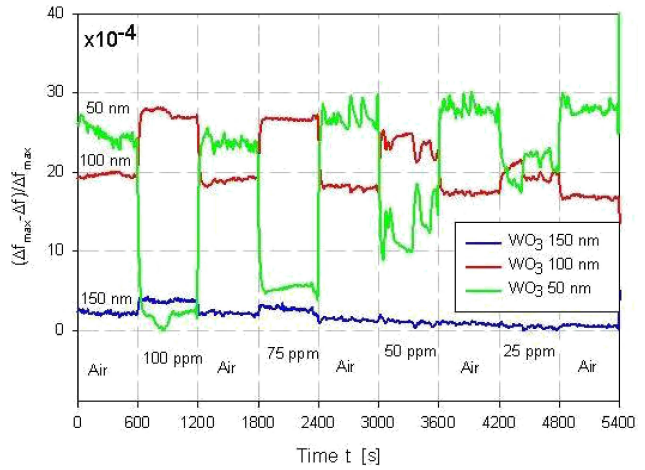
Fig. 5. Relative changes of the response of a sensor normed to maximum differential frequency for each \text{WO}_3 + \text{Pd} : 50, 100, 150 nm CO gas (25, 50, 75, 100 ppm), in synthetic air, T = 40^\circ\text{C} .
