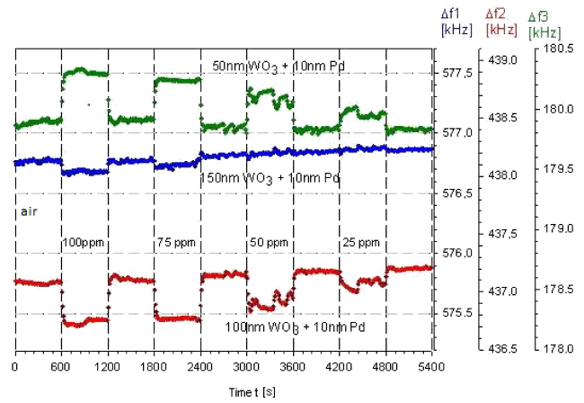
Fig. 4. Experimental results – response ( \Delta f ) sensor for thickness layers of the \text{WO}_3 + \text{Pd} : 50, 100, 150 nm CO gas (25, 50, 75, 100 ppm), T = 40^\circ\text{C} .
