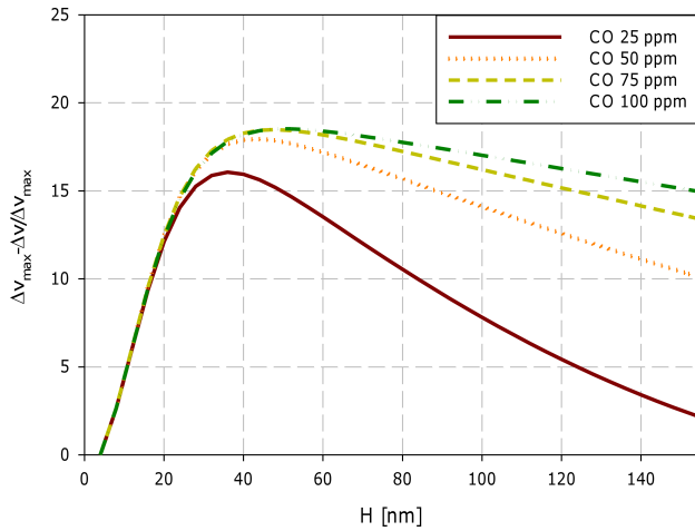
Fig. 3. Relative changes of velocity vs. sensor layer thickness – numerical results. Sensitivity coefficient a = 0.5 \text{ ppm}^{-1} , \sigma_S = 4.7 \times 10^{-7} , k = 10^8 \text{ s}^{-1} , D_K = 10^{12} \text{ nm}^2 \text{ s}^{-1} , E_g = 2.7 \text{ eV} , M = 28 \text{ g/mol} (CO) (HEJCZYK, URBAŃCZYK, 2013).
