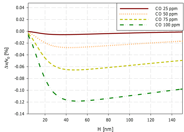
Fig. 10. SAW velocity changes of CO vs. thickness in the layer from 0 to 150 nm in synthetic air in 40^\circ\text{C} at concentration: 25, 50, 75, 100 ppm. Calculations were performed for the sensitivity coefficient a = 0.5 \text{ ppm}^{-1} , \sigma_S = 4.7 \times 10^{-7} \text{ S} , k = 10^8 \text{ s}^{-1} , D_K = 10^{12} \text{ nm}^2 \text{ s}^{-1} , E_g = 2.7 \text{ eV} , M = 28 \text{ g/mol} , r = 2 \text{ nm} (CO).
