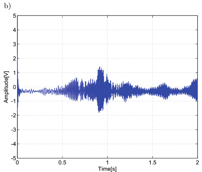
Fig. 18. Experimental results – the plate response for chirp signal (from 10 Hz to 500 Hz) excitation; a) open loop control system, b) close loop control system.
