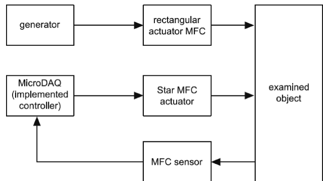
Fig. 14. Vibration reduction system used during the simulation controller operation.
