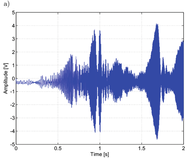
Fig. 15. Plate response for 190 Hz periodic excitation; 0–2 s open loop control system, 2–4 s close loop control system.
