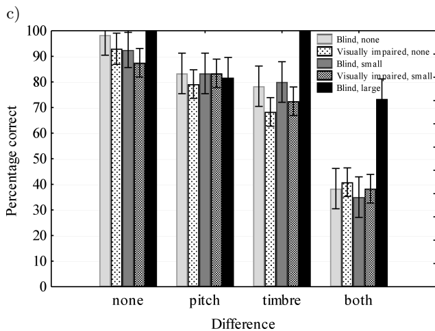
Fig. 2. Means and standard errors of percentage of correct answers in the pitch-timbre categorization task for: a) three groups of blind subjects (none, small, substantial (large) musical experience) and corresponding sighted reference groups, b) two groups of visually impaired subjects (none, small musical experience) and corresponding sighted reference groups, c) three groups of blind subjects (none, small, substantial (large) musical experience) and two groups of visually impaired subjects (none or small musical experience).
