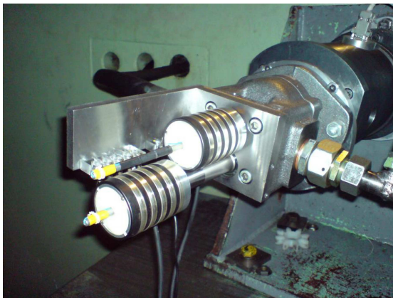
Fig. 7. Pump PGP 620 on the test bench (Wrocław University of Technology).
