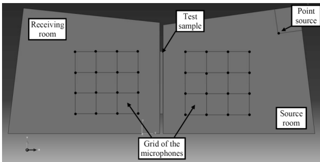
Fig. 6. Two-dimensional numerical FE model of acoustic laboratory of Fig. 2 (grid visualizes microphones' distribution in both acoustic chambers).
