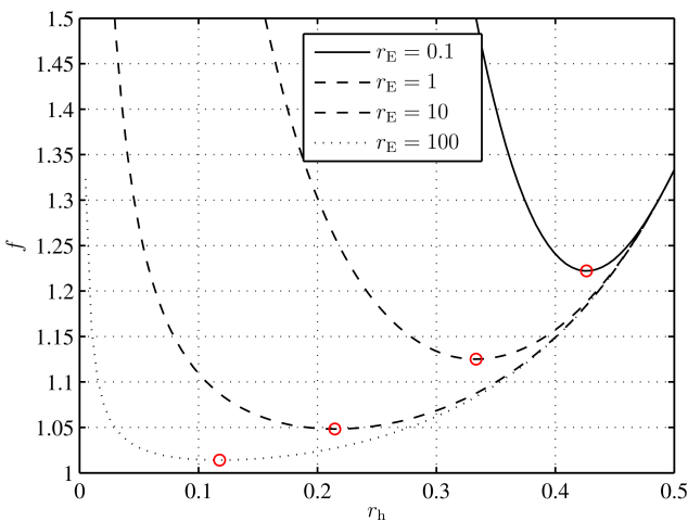
Fig. 7. Functio f versus thickness ratio r_h for various r_E .
