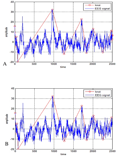
Fig.5. Knots in EEG signal for Multiplication task before and after reduction A. Before reduction, B. After reduction
