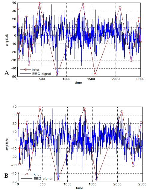
Fig.6. Knots in EEG signal for Letter Composing task before and after reduction A. Before reduction, B. After reduction
