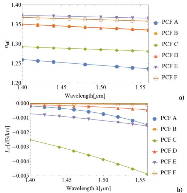
Fig. 2. (a) Effective index n_{\text{eff}} and (b) Confinement factor loss L_c for different PCF configurations.
