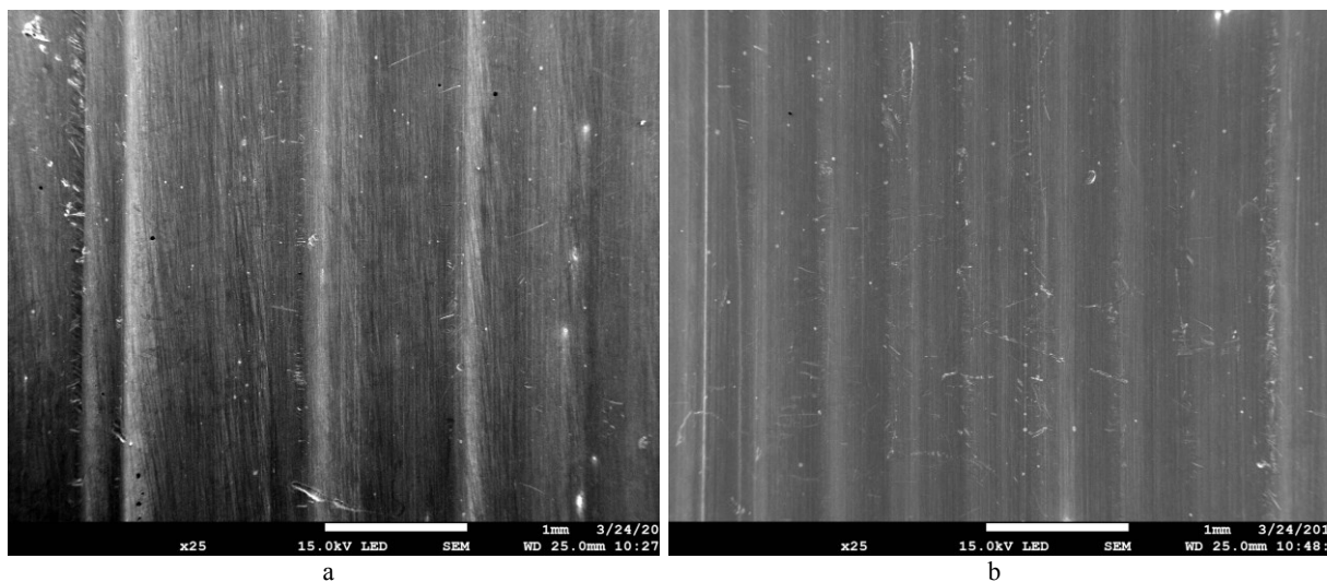
Fig. 3. SEM images of the cast steel after the Miller test, a) non-modified cast steel, b) modified cast steel
