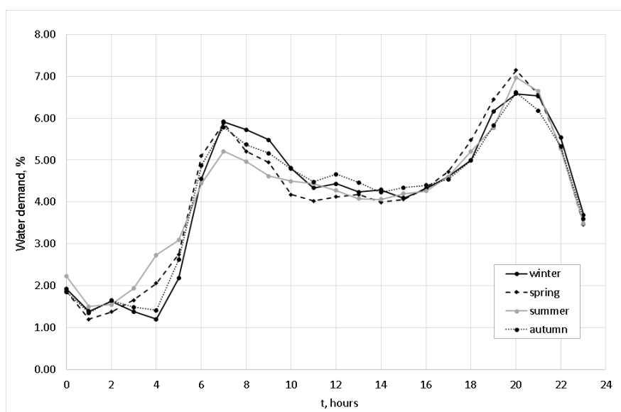
Fig. 4. Mean hourly water demand on working days during each season; source: own study
