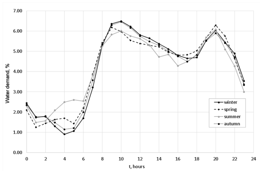
Fig. 5. Mean hourly water demand on days off work during each season; source: own study
