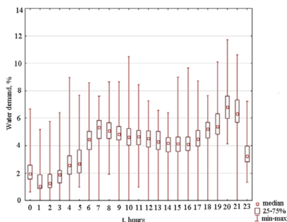
Fig. 2. A distribution of an hourly water demand on working days during a summer; source: own study
