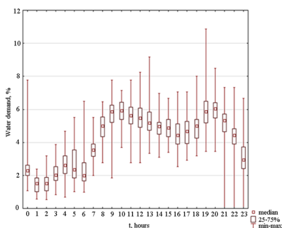
Fig. 3. A distribution of an hourly water demand on days off work during a summer; source: own study
