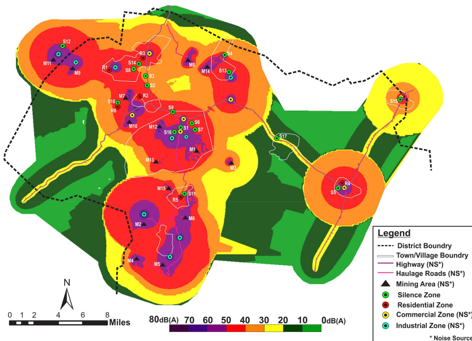
Fig. 5. Noise contour map representing predicted noise index during the day-night time.
