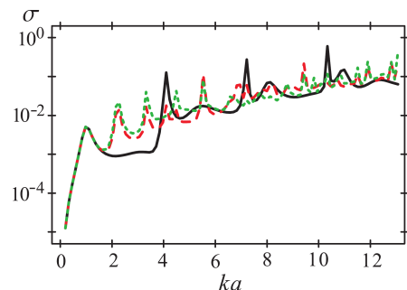
Fig. 11. The radiation efficiency \sigma as a function of the normalized angular frequency ka for H/a = 1 , l_x/a = 0.1 , l_y/a = 0.05 and W = 15 . The line keys: solid – the piston location I, dashed – the piston location II and dotted – the piston location III.
