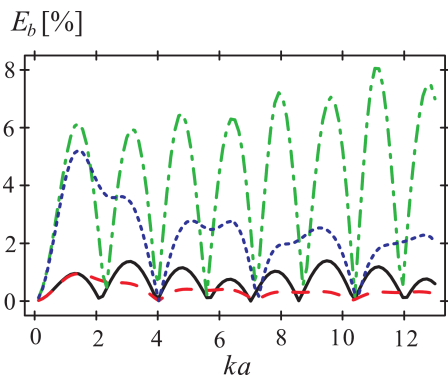
Fig. 9. The relative error E_b given by Eq. (46) as a function of the normalized angular frequency ka for l_x/a = 0.1 , l_y/a = 0.05 and W = 15 . The line keys: solid – the piston location I and H/a = 0.01 , dashed – the piston location II and H/a = 0.01 , dashed-dotted – the piston location I and H/a = 0.05 and dotted – the piston location II and H/a = 0.05 .
