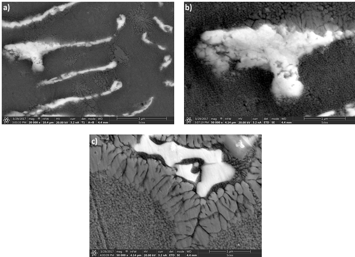
Fig. 10. Microstructure of fusion zone: a) arms of Chinese script carbide; b) fine \gamma' precipitates adjacent to the carbide; c) regular shape carbide inside eutectic \gamma/\gamma' . SEM
