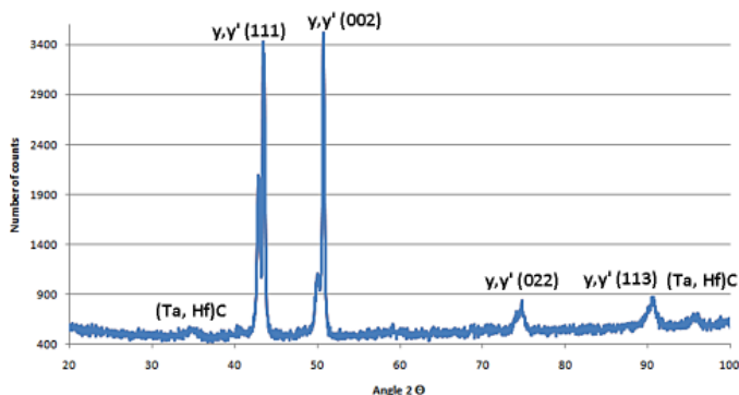
Fig. 6. X-ray spectrum of MAR-M247. Radiation Cu K_{\alpha}
