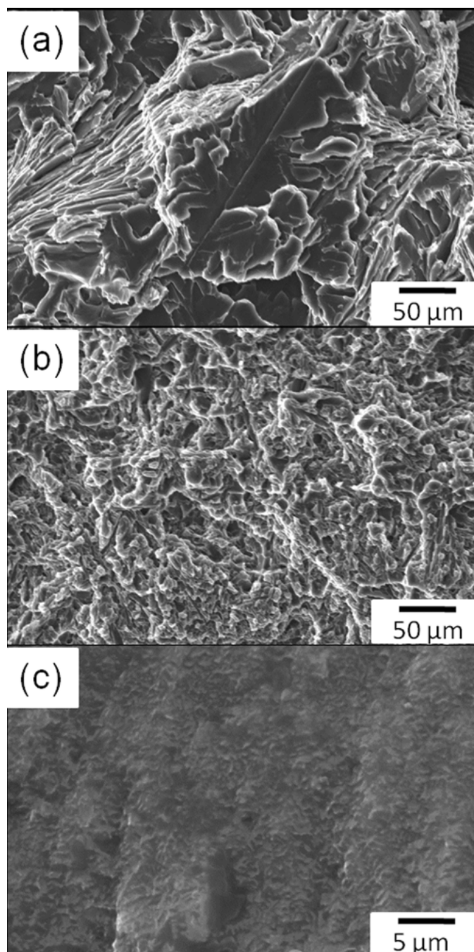
Fig. 6. SEM fractographs showing the fracture surface of (a) IMed, (b) ARed and (c) MS alloys
