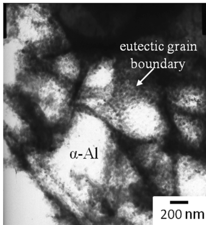
Fig. 3. TEM micrograph of the melt-spun alloy
