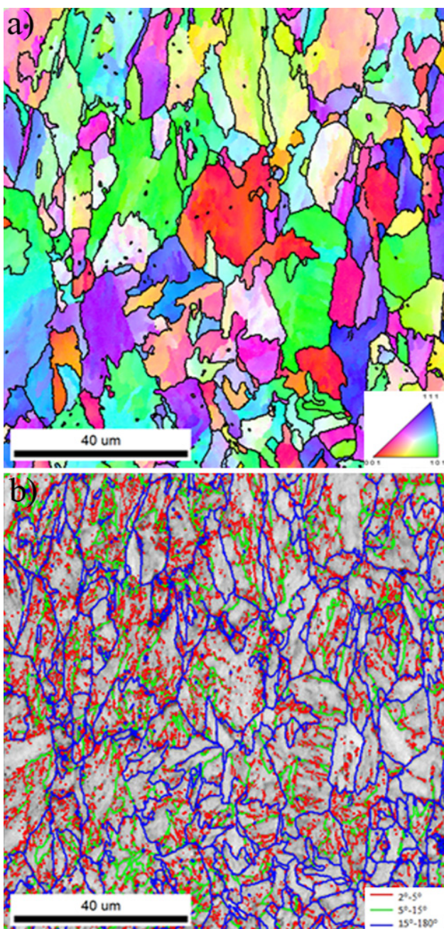
Fig. 9. EBSD analysis results for 703 K austempered specimen: (a) IPF; (b) boundary misorientation
