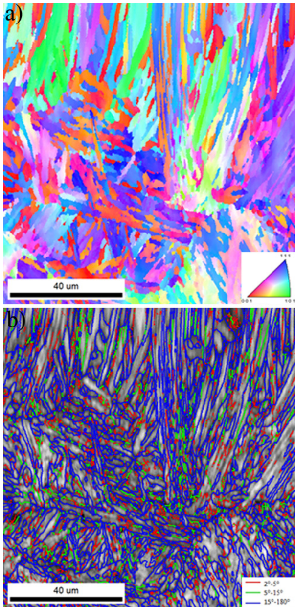
Fig. 7. EBSD analysis results for DQT-S specimen: (a) IPF; (b) boundary misorientation
