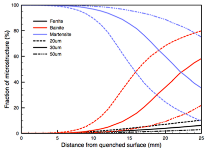
Fig. 4. Fractions of different microstructural components below the quenched surface simulated by JMatPro with various prior austenite grain sizes
