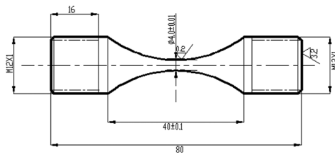
(a) The conventional frequency specimen dimensions
