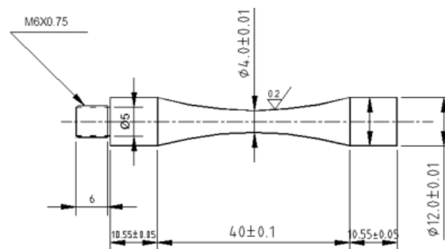
(b) The ultrasonic frequency specimen dimensions
