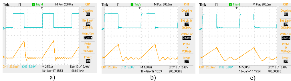
Fig. 8 Gate-source voltage (top) and inductor current (bottom) of BUCK converter(transistor APP9962, diode IDD03SG60C) in DCM for different frequencies: a – f_s = 100 kHz, b – f_s = 200 kHz; c – f_s = 400 kHz
