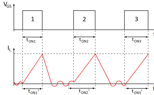
Fig. 5. Intervals of control signal V_{GS} and inductor current I_L in DCM
