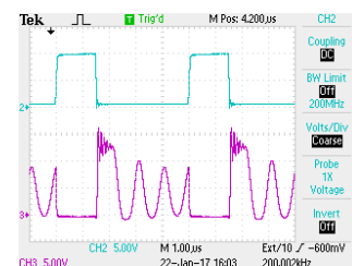
Fig. 4. Gate-source voltage (top) and drain-source voltage (bottom) of BUCK converter working in DCM
