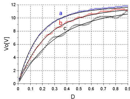
Fig. 7. Output voltage of a BUCK converter (APP9962 transistor, IDD03SG60C diode) in DCM for different frequencies: a – f_s = 100 kHz; b – f_s = 200 kHz; c – f_s = 400 kHz; solid line – calculated from Eq. (4); dotted line – measured value
