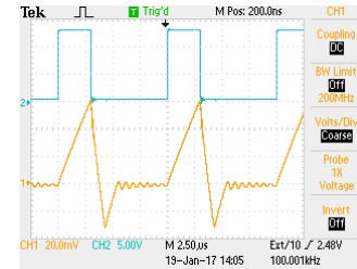
Fig. 12. Gate-source voltage (top) and inductor current (bottom) of a BUCK converter which uses transistor AP9962 ( C_T = 250 pF) and diode 1N4007 ( C_D = 4.5 pF, t_{rr} = 1 µs)
