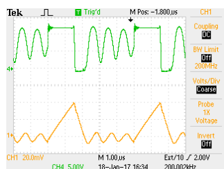
Fig. 2. Diode voltage (top) and inductor current (bottom) of BUCK converter working in DCM
