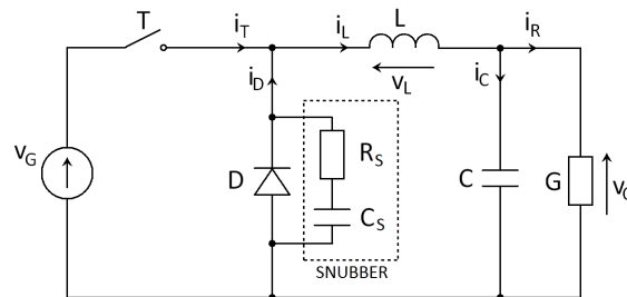
Fig. 15. Snubber circuit in BUCK converter
