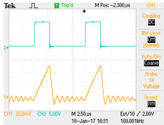
Fig. 10. Gate-source voltage (top) and inductor current (bottom) of a BUCK converter which uses transistor IRFZ44 ( C_T = 650 pF) and diode IDD03SG60C ( C_D = 30 pF)
