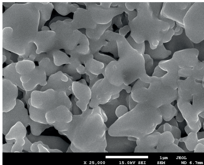
Fig. 2. SEM micrographs of the LSCF electrode
