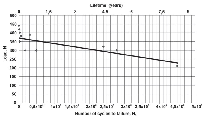
Fig. 8 The load-cycle diagram the fatigue limit of the implantological system with the zirconia abutment
