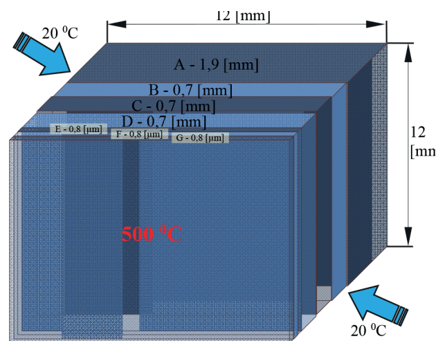
Fig. 1. Dimensioning model in SD section
