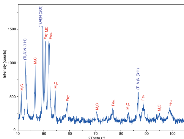
Fig. 8. Diffraction patterns of the steel matrix +(Ti,Al)N variant of PVD coated high-speed steel matrix composite
