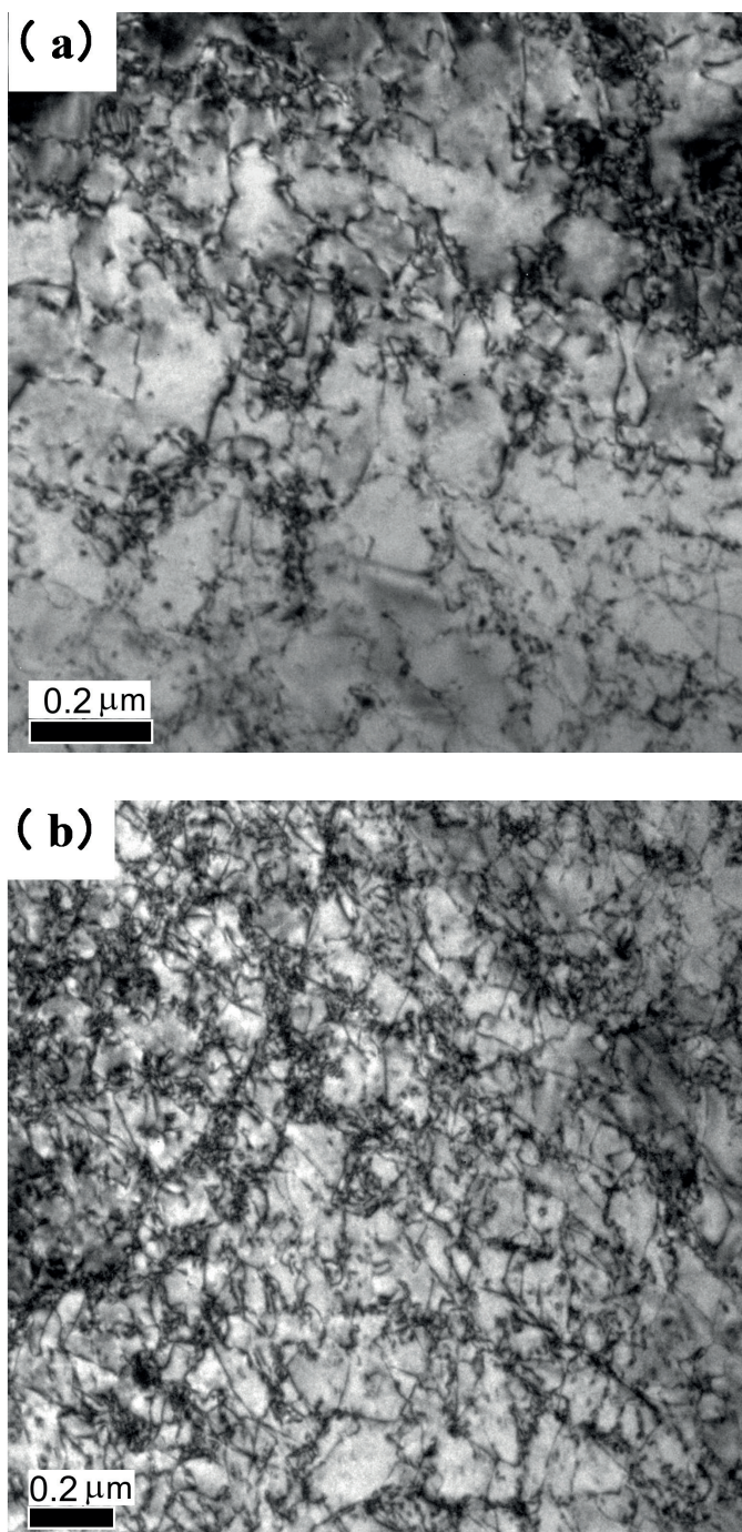
Fig. 3. Influence of prestrain on the dislocation structure in cold rolled low carbon steel after baking at 170°C for 20 min. (a) 2%, (b) 5%, and (c) 10%
