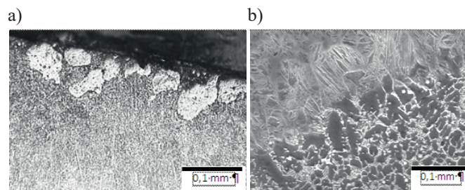
Fig. 8. The cross-section of laser surface alloyed of X2CrMoV12-28 steel at laser beam power of 1.6 kW, a) the top layer after alloying with TaC powder, b) the fusion line after alloying with TiC powder
