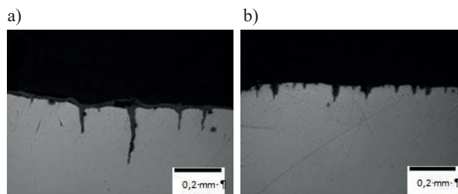
Fig. 9. The cracks on the surface layer cross section after thermal fatigue test of X40CrMoV5-1 steel after laser surface alloying with WC powder with the laser beam power of a) 1.6 kW and b) 2.0 kW
