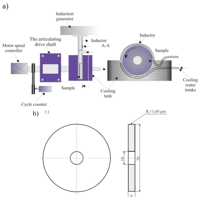
Fig. 1. a) Scheme of the stand for thermal fatigue investigations, b) Shape and size in [mm] of the sample for thermal fatigue investigations with the correspond roughness of the surface in [µm]
