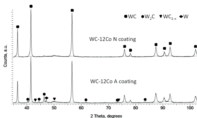
Fig. 8. XRD patterns of HVOF sprayed WC-12Co (N) and WC-12Co (A) coatings
