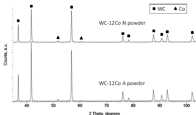
Fig. 7. XRD patterns of WC-12Co (N) and WC-12Co (A) powders
