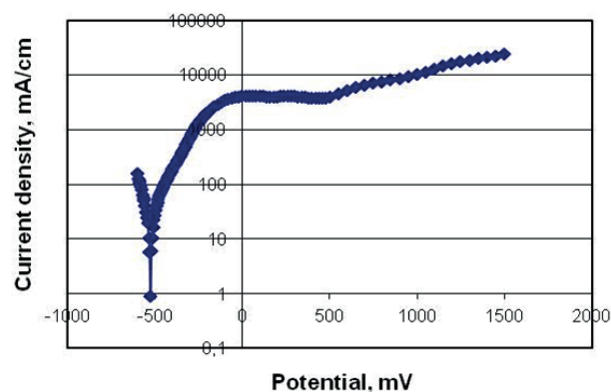
Fig. 14. Polarization curve for WC-12Co (A) coating
